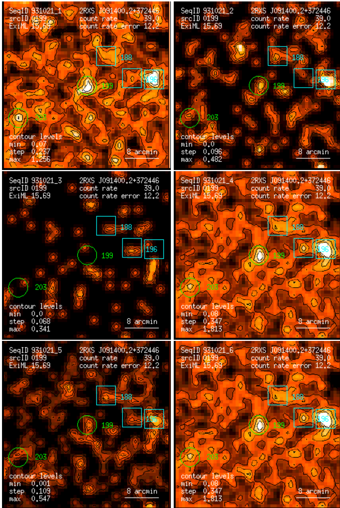
Figure 199: RASS 931021: detection 0199: band rate images, Gaussian filter: (1) PSPC channels 11 – 41, (2) 52 – 90, (3) 91 – 201, (4) 11 – 235, (5) 52 – 201, (6) 11 – 201. Broad band rates in counts/ks. Band rate contour levels in counts/ks/arcmin 2 .
