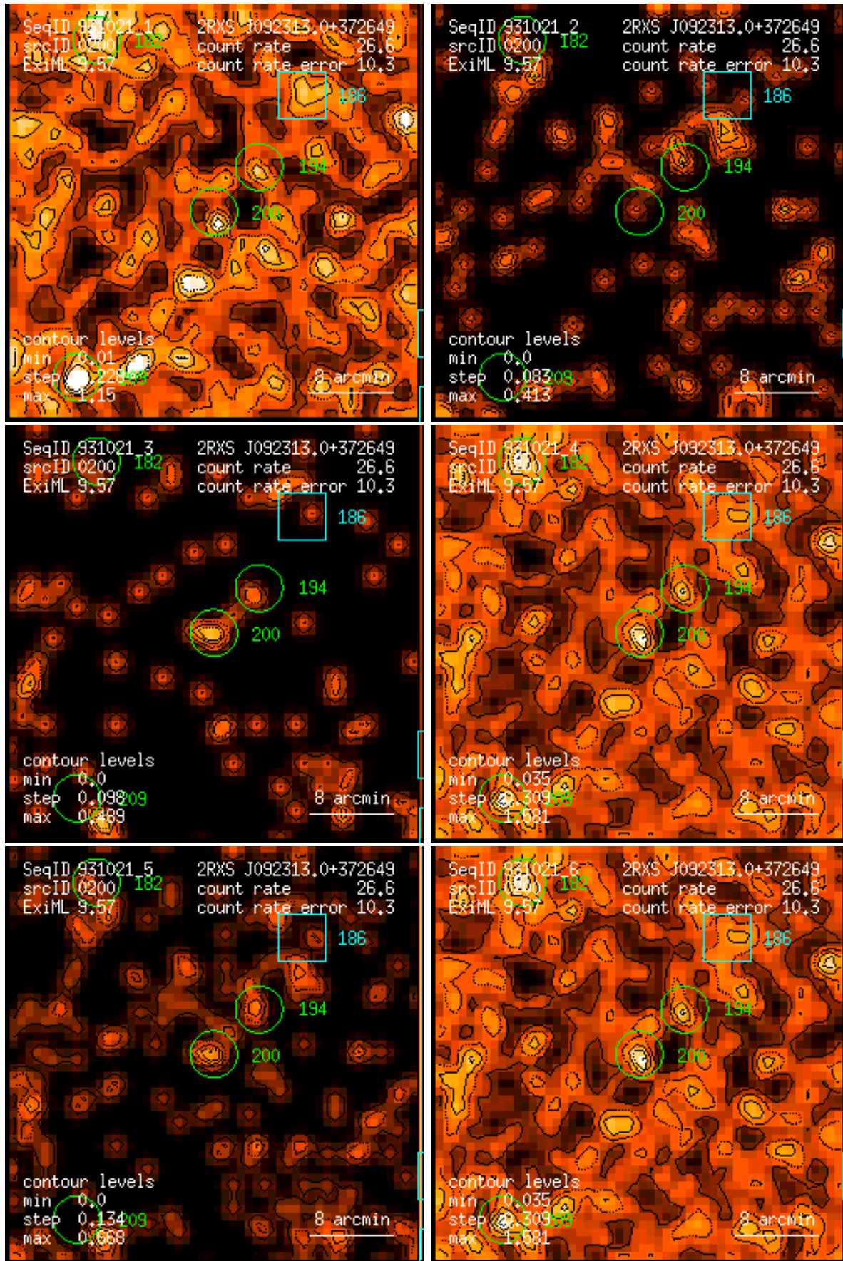
Figure 200: RASS 931021: detection 0200: band rate images, Gaussian filter: (1) PSPC channels 11 – 41, (2) 52 – 90, (3) 91 – 201, (4) 11 – 235, (5) 52 – 201, (6) 11 – 201. Broad band rates in counts/ks. Band rate contour levels in counts/ks/arcmin 2 .
