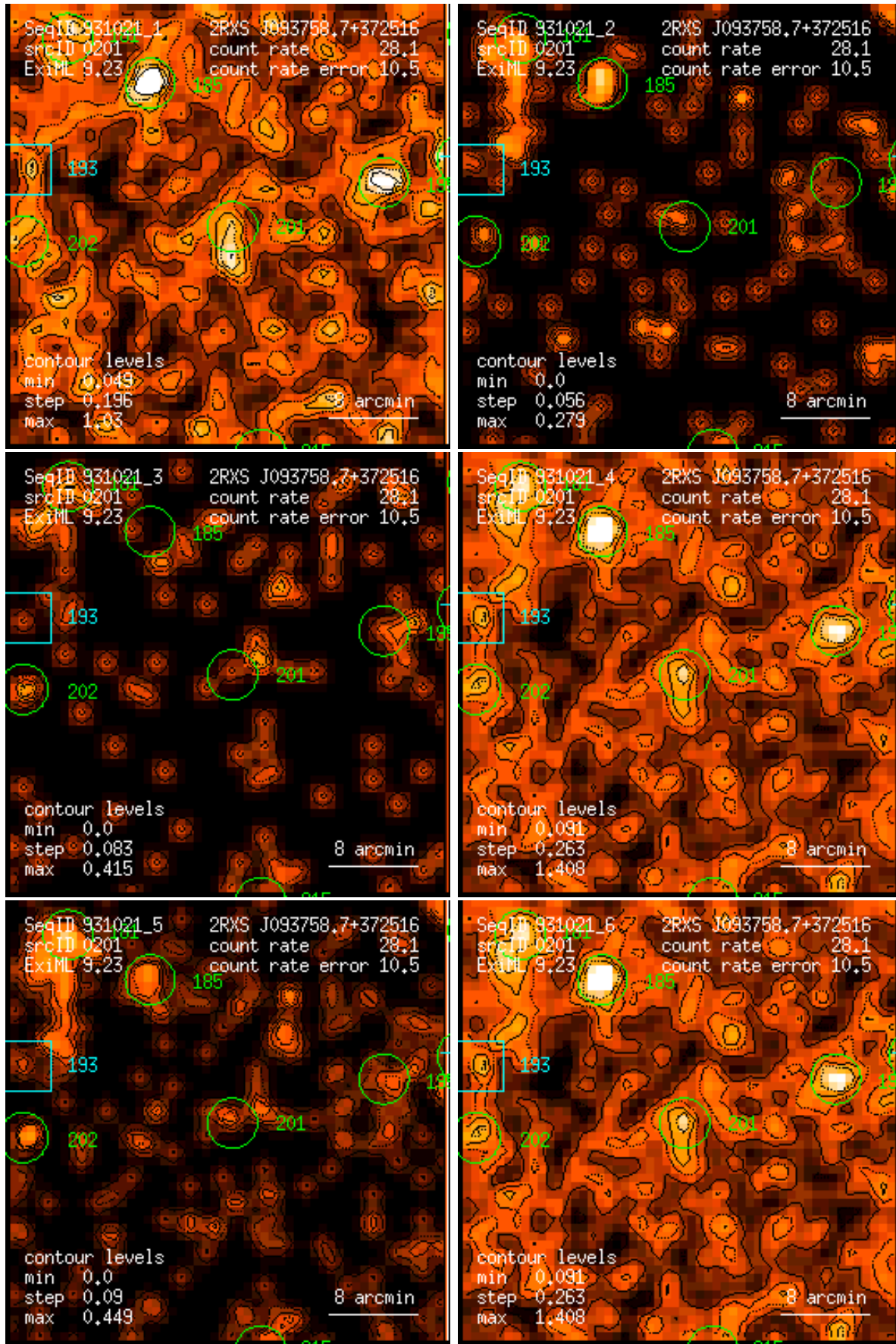
Figure 201: RASS 931021: detection 0201: band rate images, Gaussian filter: (1) PSPC channels 11 – 41, (2) 52 – 90, (3) 91 – 201, (4) 11 – 235, (5) 52 – 201, (6) 11 – 201. Broad band rates in counts/ks. Band rate contour levels in counts/ks/arcmin 2 .
