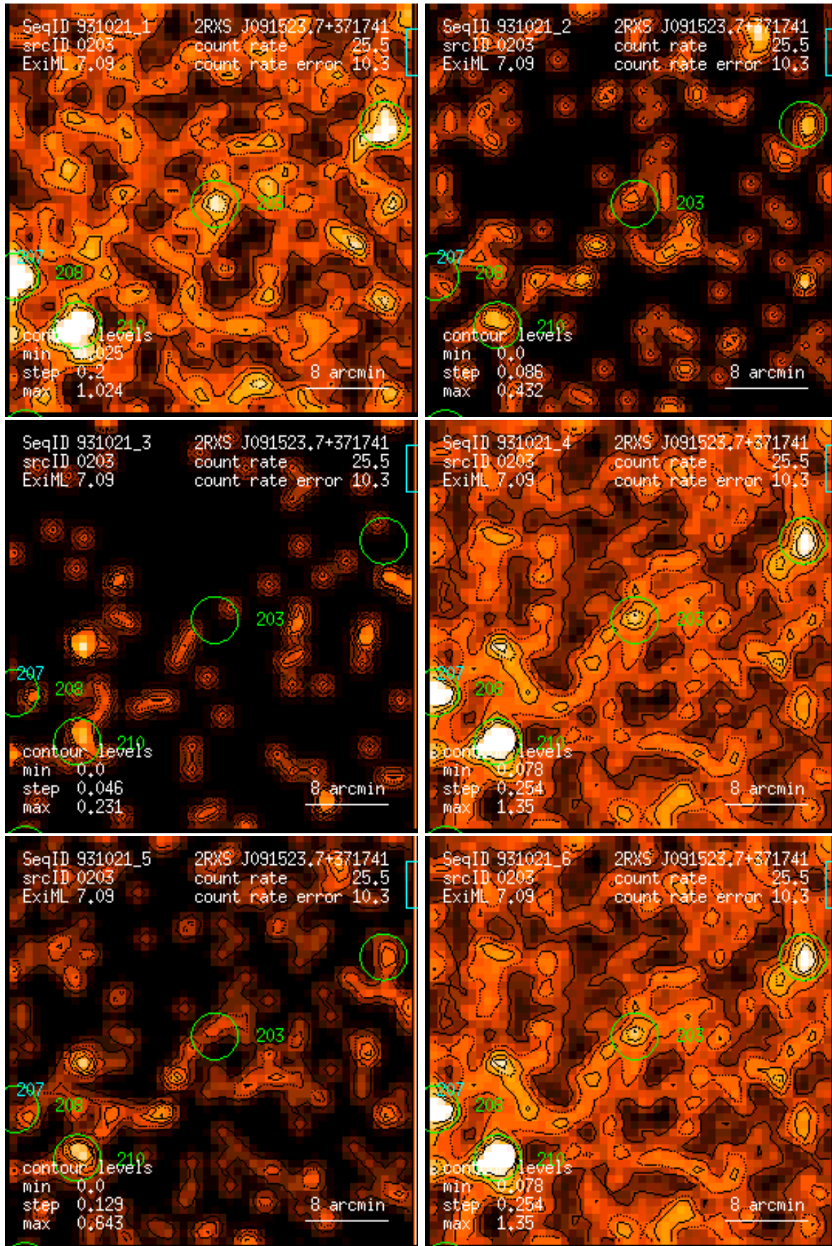
Figure 203: RASS 931021: detection 0203: band rate images, Gaussian filter: (1) PSPC channels 11 – 41, (2) 52 – 90, (3) 91 – 201, (4) 11 – 235, (5) 52 – 201, (6) 11 – 201. Broad band rates in counts/ks. Band rate contour levels in counts/ks/arcmin 2 .
