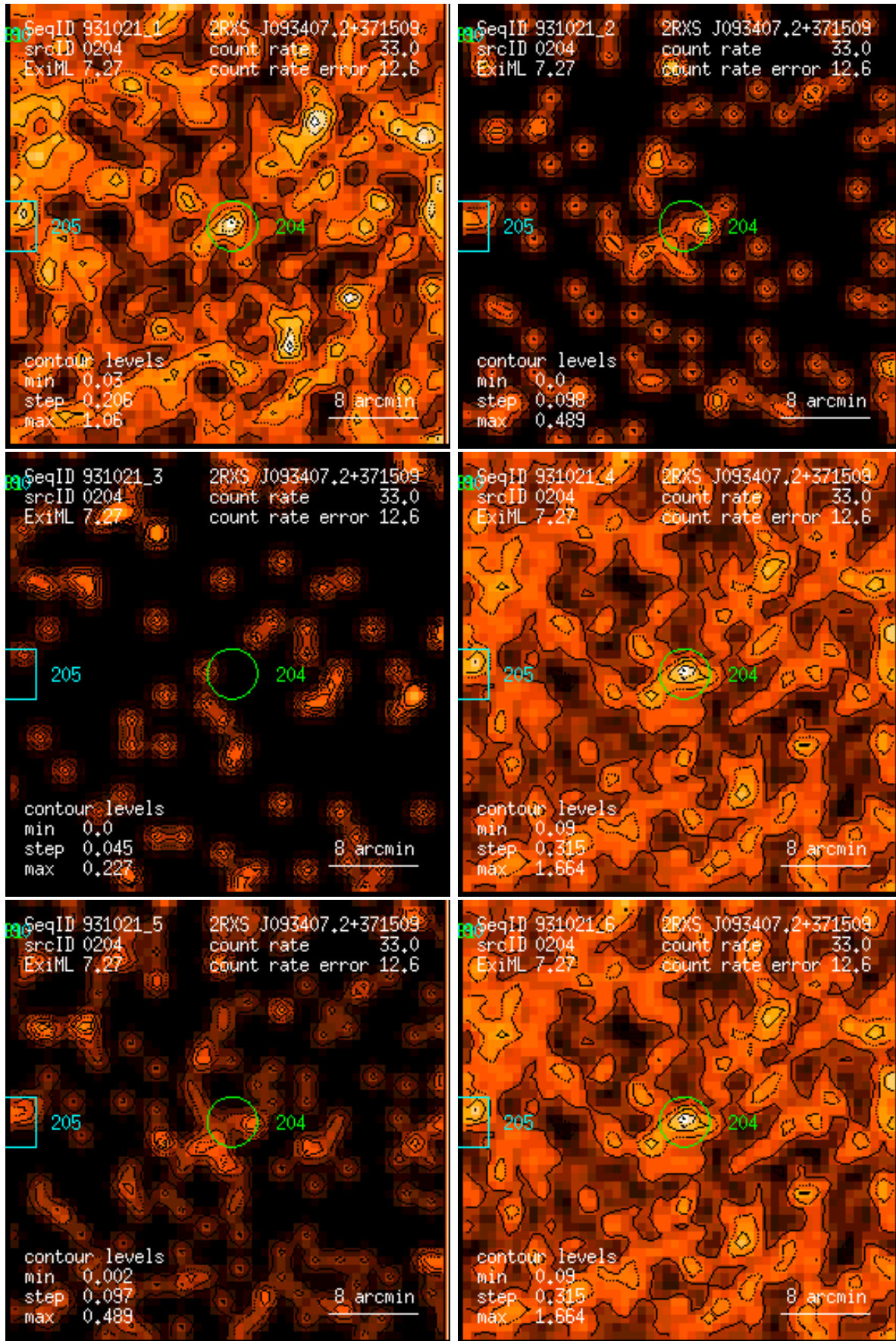
Figure 204: RASS 931021: detection 0204: band rate images, Gaussian filter: (1) PSPC channels 11 – 41, (2) 52 – 90, (3) 91 – 201, (4) 11 – 235, (5) 52 – 201, (6) 11 – 201. Broad band rates in counts/ks. Band rate contour levels in counts/ks/arcmin 2 .
