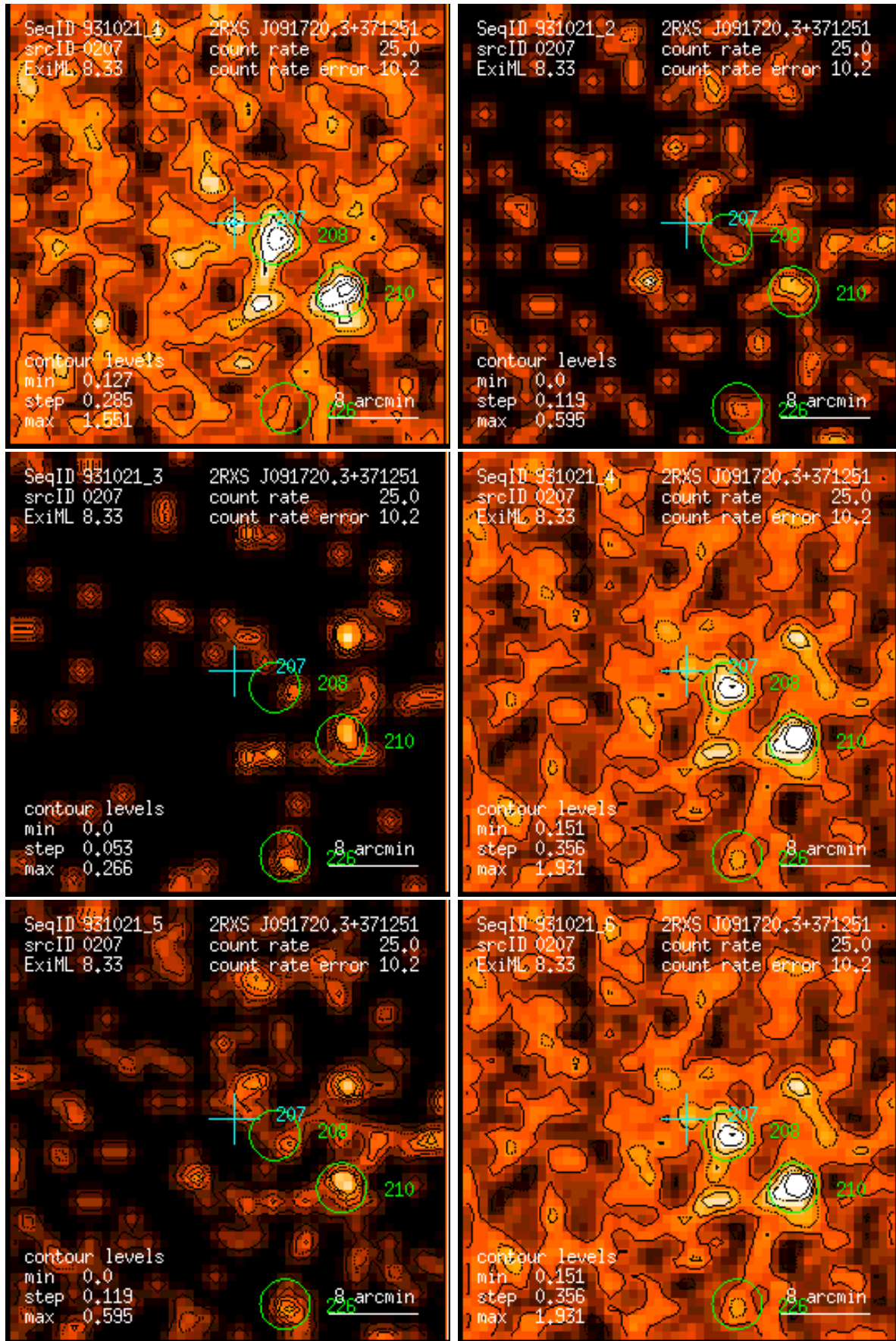
Figure 207: RASS 931021: detection 0207: band rate images, Gaussian filter: (1) PSPC channels 11 – 41, (2) 52 – 90, (3) 91 – 201, (4) 11 – 235, (5) 52 – 201, (6) 11 – 201. Broad band rates in counts/ks. Band rate contour levels in counts/ks/arcmin 2 .
