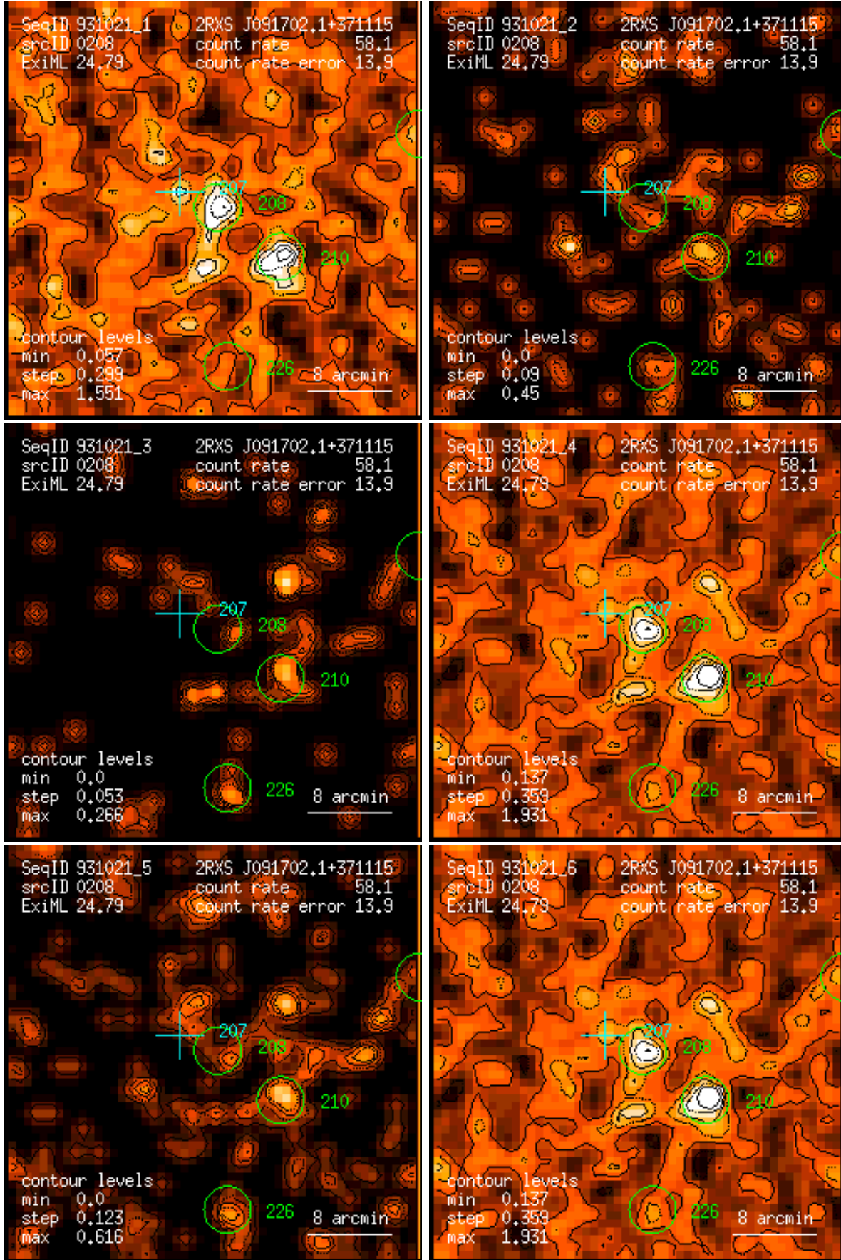
Figure 208: RASS 931021: detection 0208: band rate images, Gaussian filter: (1) PSPC channels 11 – 41, (2) 52 – 90, (3) 91 – 201, (4) 11 – 235, (5) 52 – 201, (6) 11 – 201. Broad band rates in counts/ks. Band rate contour levels in counts/ks/arcmin 2 .
