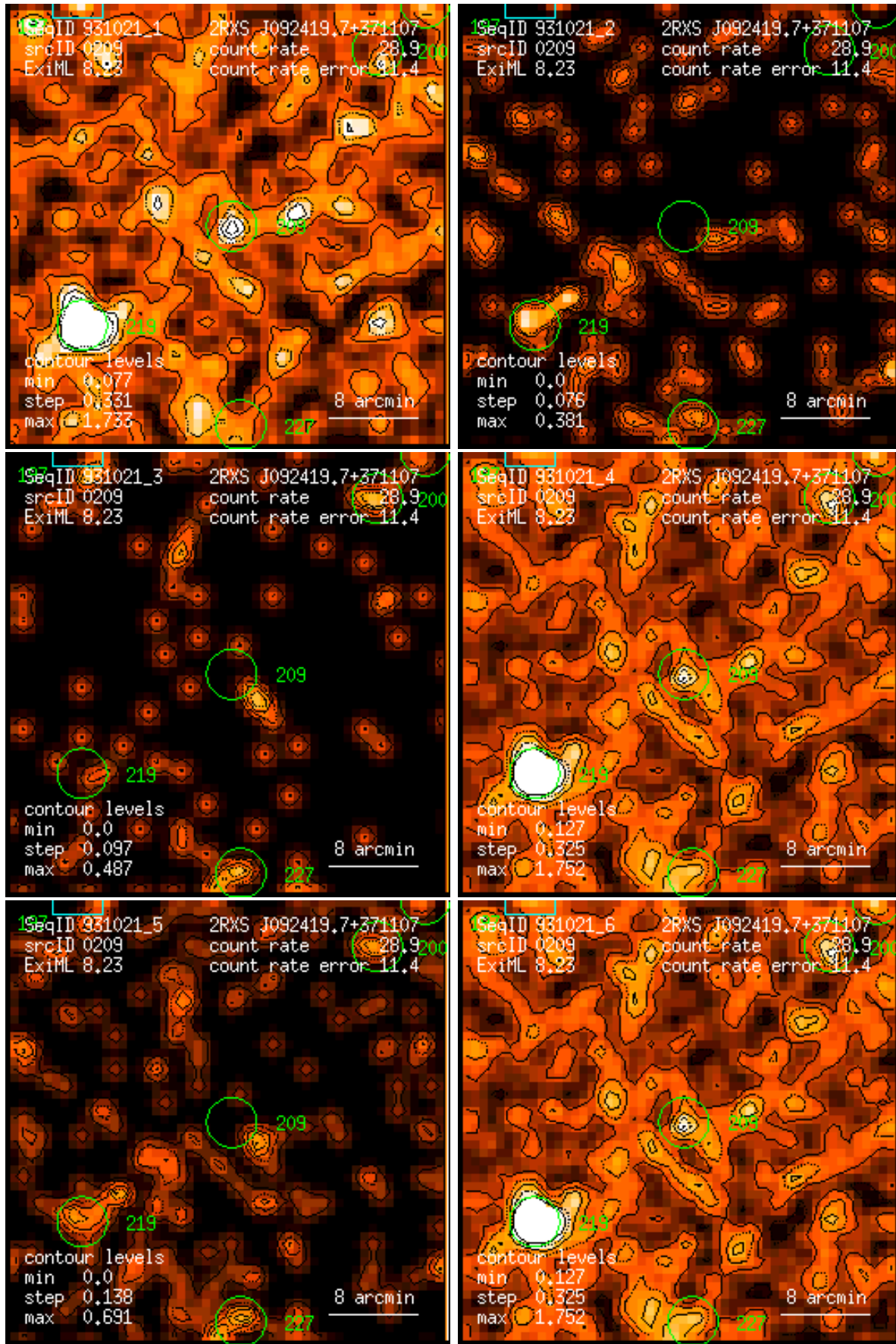
Figure 209: RASS 931021: detection 0209: band rate images, Gaussian filter: (1) PSPC channels 11 – 41, (2) 52 – 90, (3) 91 – 201, (4) 11 – 235, (5) 52 – 201, (6) 11 – 201. Broad band rates in counts/ks. Band rate contour levels in counts/ks/arcmin 2 .
