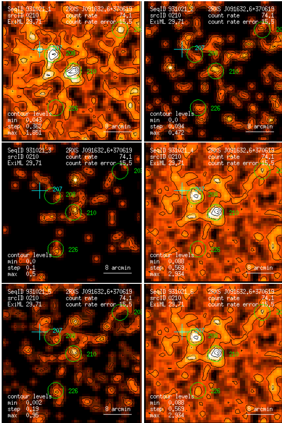
Figure 210: RASS 931021: detection 0210: band rate images, Gaussian filter: (1) PSPC channels 11 – 41, (2) 52 – 90, (3) 91 – 201, (4) 11 – 235, (5) 52 – 201, (6) 11 – 201. Broad band rates in counts/ks. Band rate contour levels in counts/ks/arcmin 2 .
