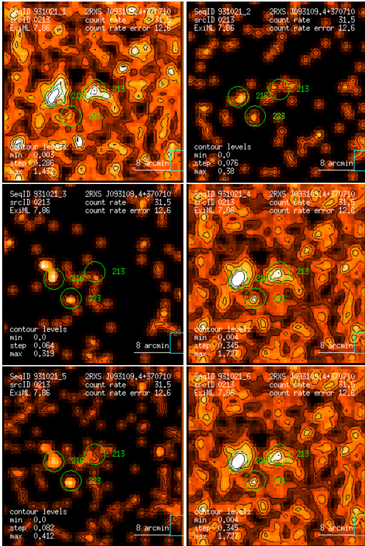
Figure 213: RASS 931021: detection 0213: band rate images, Gaussian filter: (1) PSPC channels 11 – 41, (2) 52 – 90, (3) 91 – 201, (4) 11 – 235, (5) 52 – 201, (6) 11 – 201. Broad band rates in counts/ks. Band rate contour levels in counts/ks/arcmin 2 .
