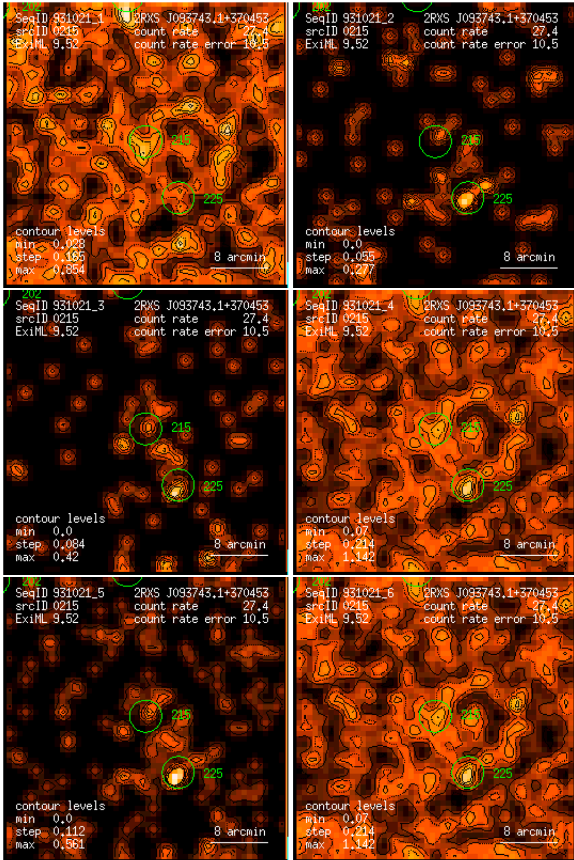
Figure 215: RASS 931021: detection 0215: band rate images, Gaussian filter: (1) PSPC channels 11 – 41, (2) 52 – 90, (3) 91 – 201, (4) 11 – 235, (5) 52 – 201, (6) 11 – 201. Broad band rates in counts/ks. Band rate contour levels in counts/ks/arcmin 2 .
