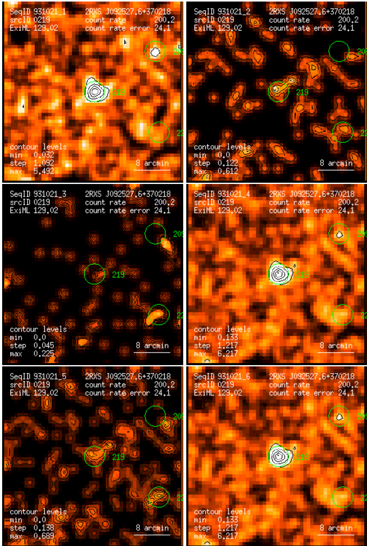
Figure 219: RASS 931021: detection 0219: band rate images, Gaussian filter: (1) PSPC channels 11 – 41, (2) 52 – 90, (3) 91 – 201, (4) 11 – 235, (5) 52 – 201, (6) 11 – 201. Broad band rates in counts/ks. Band rate contour levels in counts/ks/arcmin 2 .
