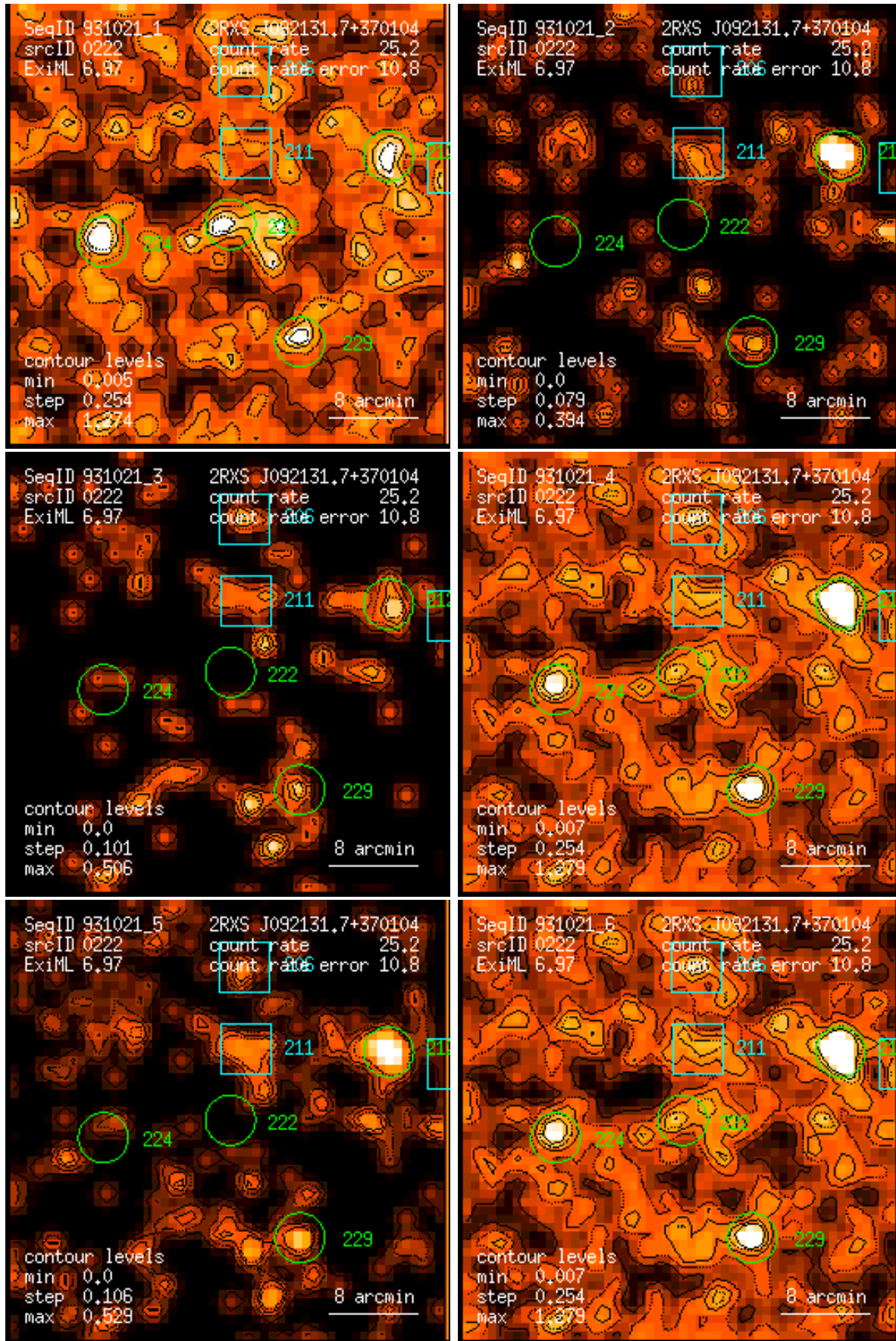
Figure 222: RASS 931021: detection 0222: band rate images, Gaussian filter: (1) PSPC channels 11 – 41, (2) 52 – 90, (3) 91 – 201, (4) 11 – 235, (5) 52 – 201, (6) 11 – 201. Broad band rates in counts/ks. Band rate contour levels in counts/ks/arcmin 2 .
