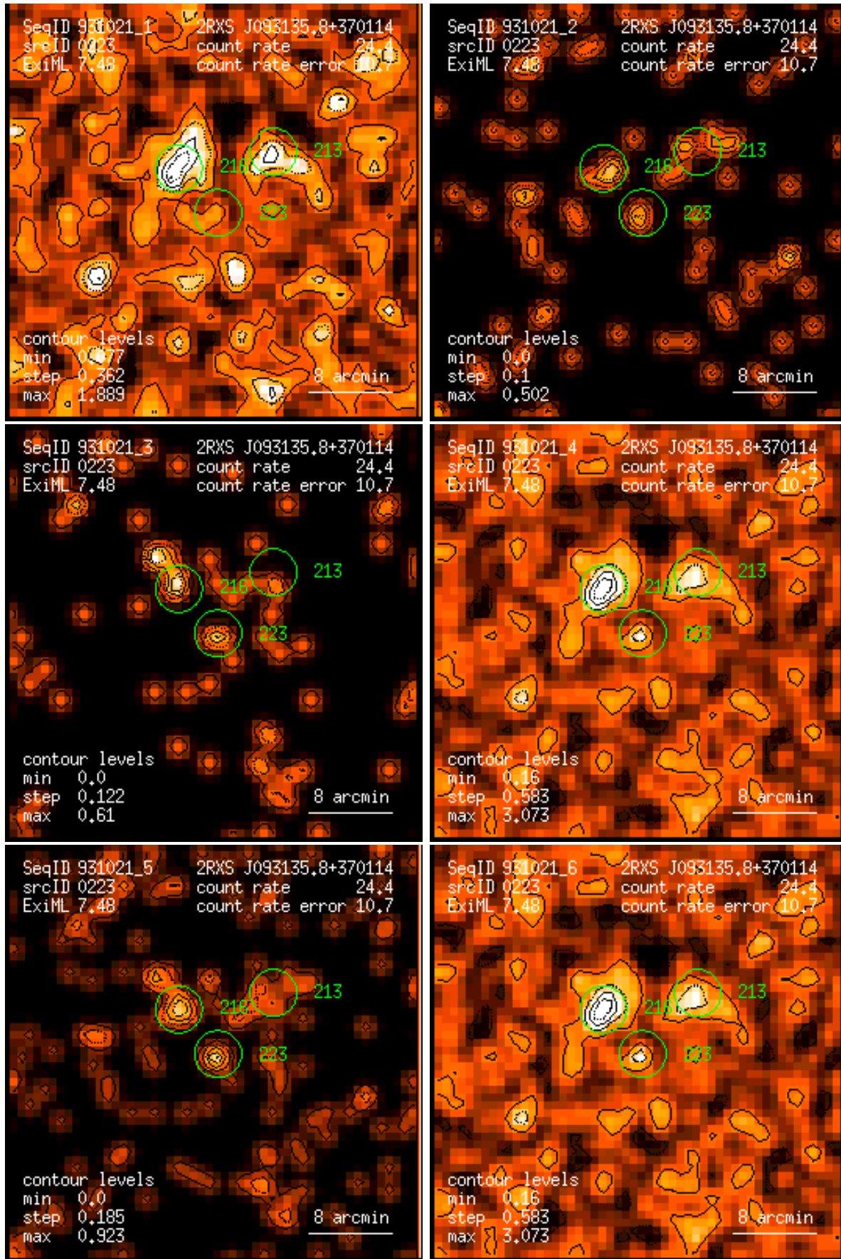
Figure 223: RASS 931021: detection 0223: band rate images, Gaussian filter: (1) PSPC channels 11 – 41, (2) 52 – 90, (3) 91 – 201, (4) 11 – 235, (5) 52 – 201, (6) 11 – 201. Broad band rates in counts/ks. Band rate contour levels in counts/ks/arcmin 2 .
