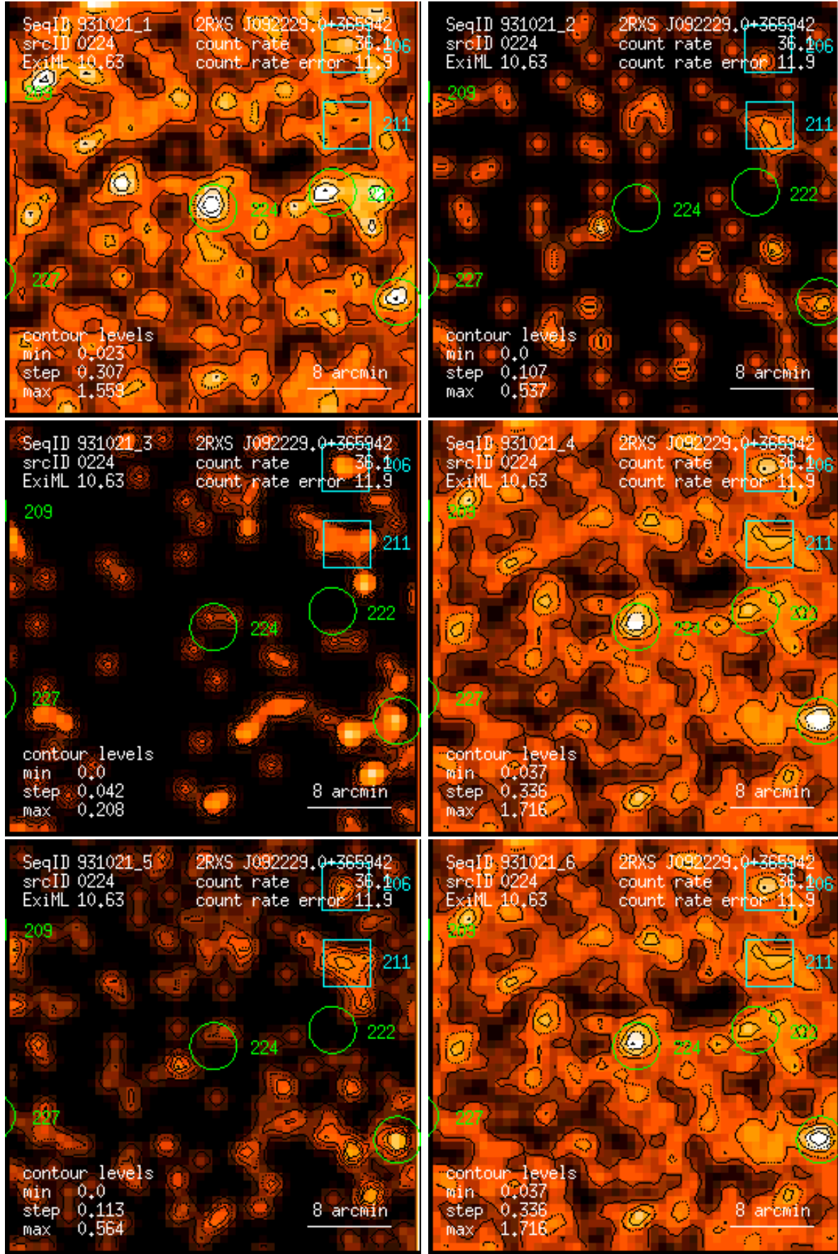
Figure 224: RASS 931021: detection 0224: band rate images, Gaussian filter: (1) PSPC channels 11 – 41, (2) 52 – 90, (3) 91 – 201, (4) 11 – 235, (5) 52 – 201, (6) 11 – 201. Broad band rates in counts/ks. Band rate contour levels in counts/ks/arcmin 2 .
