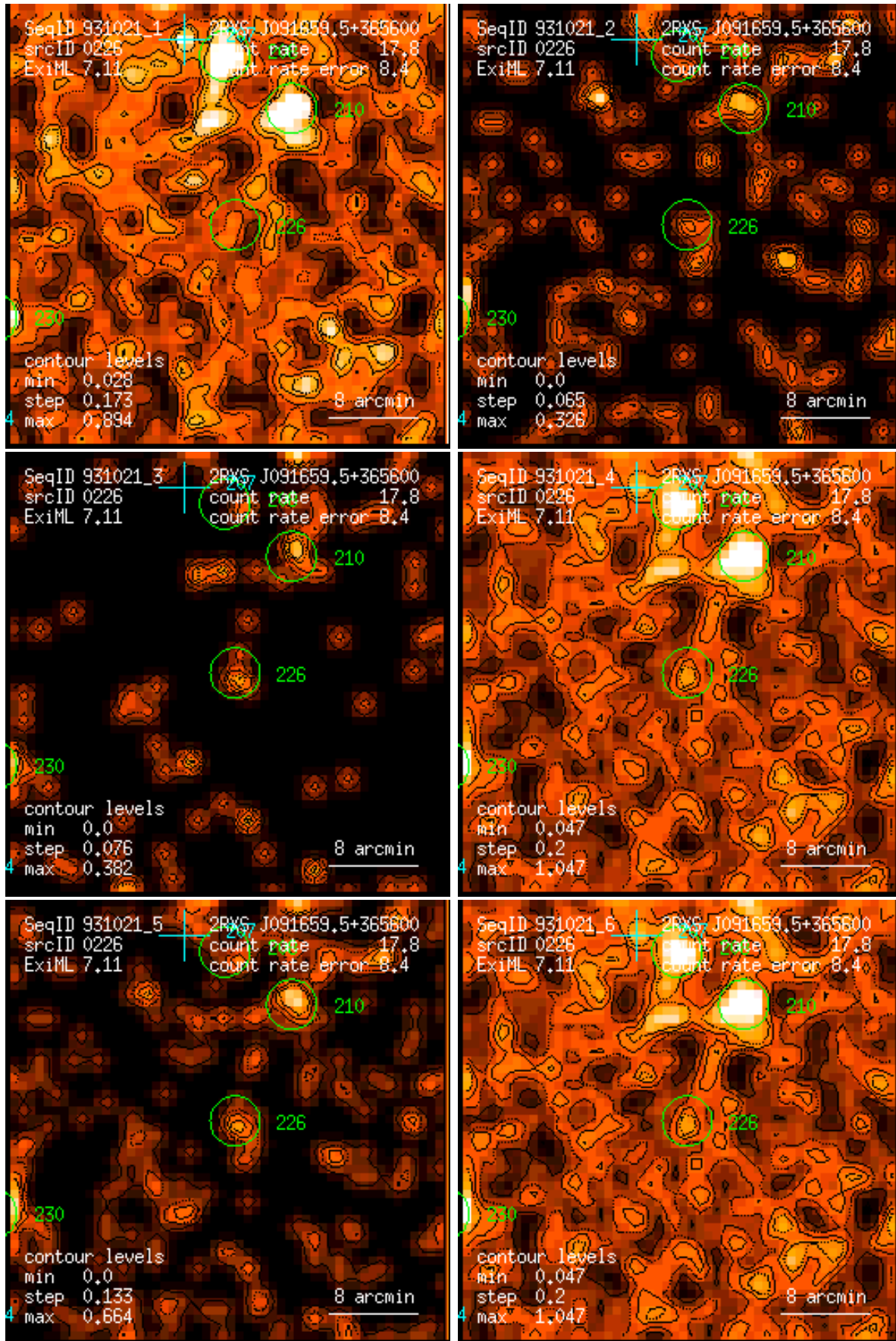
Figure 226: RASS 931021: detection 0226: band rate images, Gaussian filter: (1) PSPC channels 11 – 41, (2) 52 – 90, (3) 91 – 201, (4) 11 – 235, (5) 52 – 201, (6) 11 – 201. Broad band rates in counts/ks. Band rate contour levels in counts/ks/arcmin 2 .
