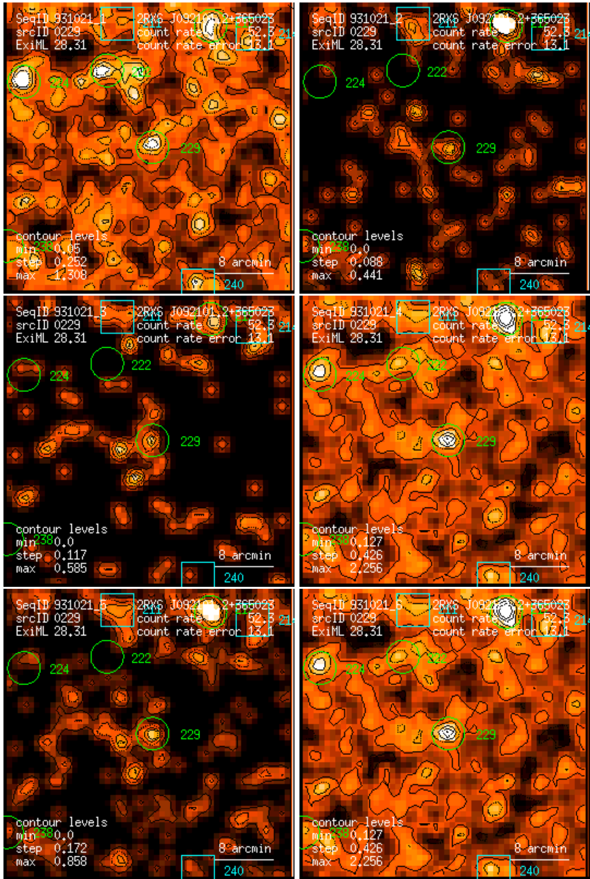
Figure 229: RASS 931021: detection 0229: band rate images, Gaussian filter: (1) PSPC channels 11 – 41, (2) 52 – 90, (3) 91 – 201, (4) 11 – 235, (5) 52 – 201, (6) 11 – 201. Broad band rates in counts/ks. Band rate contour levels in counts/ks/arcmin 2 .
