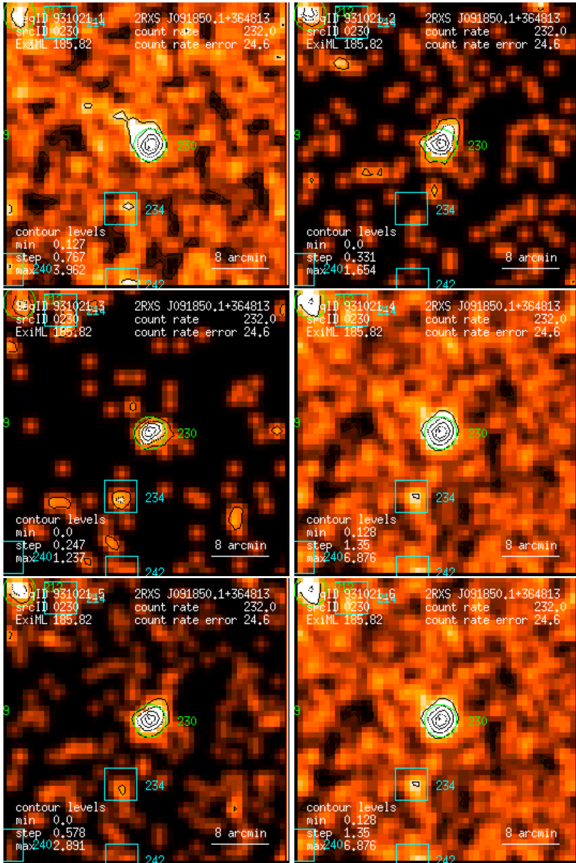
Figure 230: RASS 931021: detection 0230: band rate images, Gaussian filter: (1) PSPC channels 11 – 41, (2) 52 – 90, (3) 91 – 201, (4) 11 – 235, (5) 52 – 201, (6) 11 – 201. Broad band rates in counts/ks. Band rate contour levels in counts/ks/arcmin 2 .
