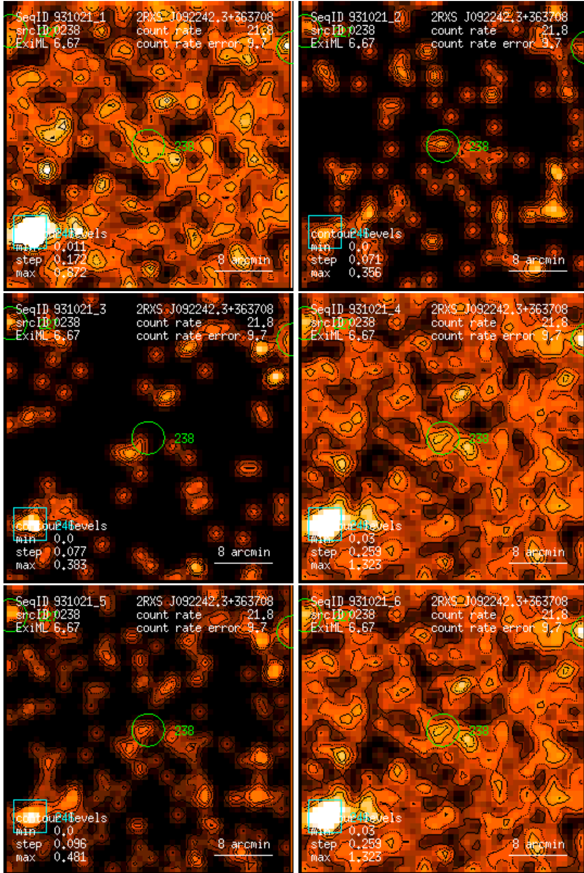
Figure 238: RASS 931021: detection 0238: band rate images, Gaussian filter: (1) PSPC channels 11 – 41, (2) 52 – 90, (3) 91 – 201, (4) 11 – 235, (5) 52 – 201, (6) 11 – 201. Broad band rates in counts/ks. Band rate contour levels in counts/ks/arcmin 2 .
