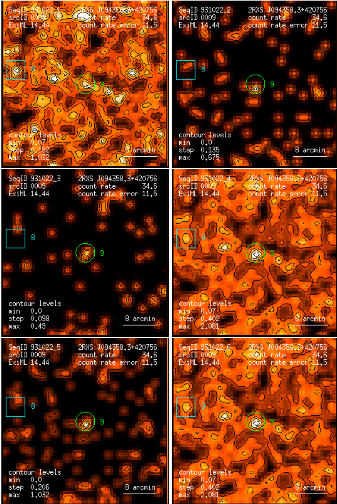
Figure 9: RASS 931022: detection 0009: band rate images, Gaussian filter: (1) PSPC channels 11 – 41, (2) 52 – 90, (3) 91 – 201, (4) 11 – 235, (5) 52 – 201, (6) 11 – 201. Broad band rates in counts/ks. Band rate contour levels in counts/ks/arcmin 2 .
