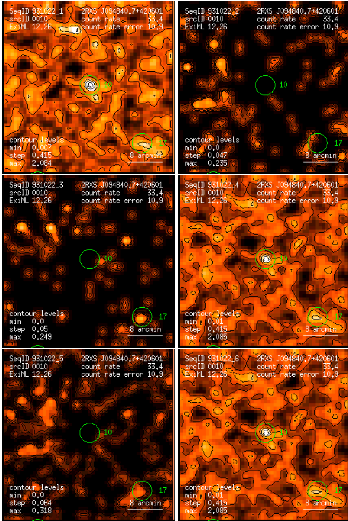
Figure 10: RASS 931022: detection 0010: band rate images, Gaussian filter: (1) PSPC channels 11 – 41, (2) 52 – 90, (3) 91 – 201, (4) 11 – 235, (5) 52 – 201, (6) 11 – 201. Broad band rates in counts/ks. Band rate contour levels in counts/ks/arcmin 2 .
