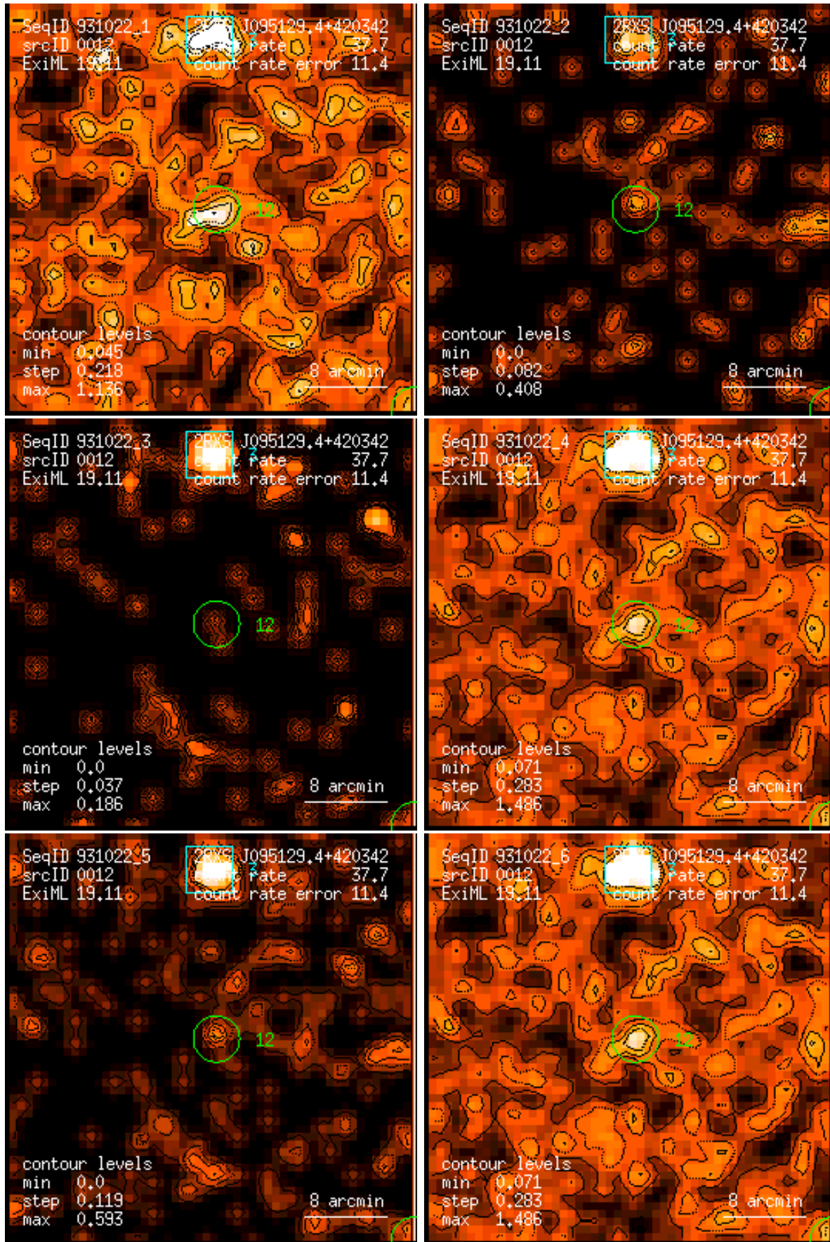
Figure 12: RASS 931022: detection 0012: band rate images, Gaussian filter: (1) PSPC channels 11 – 41, (2) 52 – 90, (3) 91 – 201, (4) 11 – 235, (5) 52 – 201, (6) 11 – 201. Broad band rates in counts/ks. Band rate contour levels in counts/ks/arcmin 2 .
