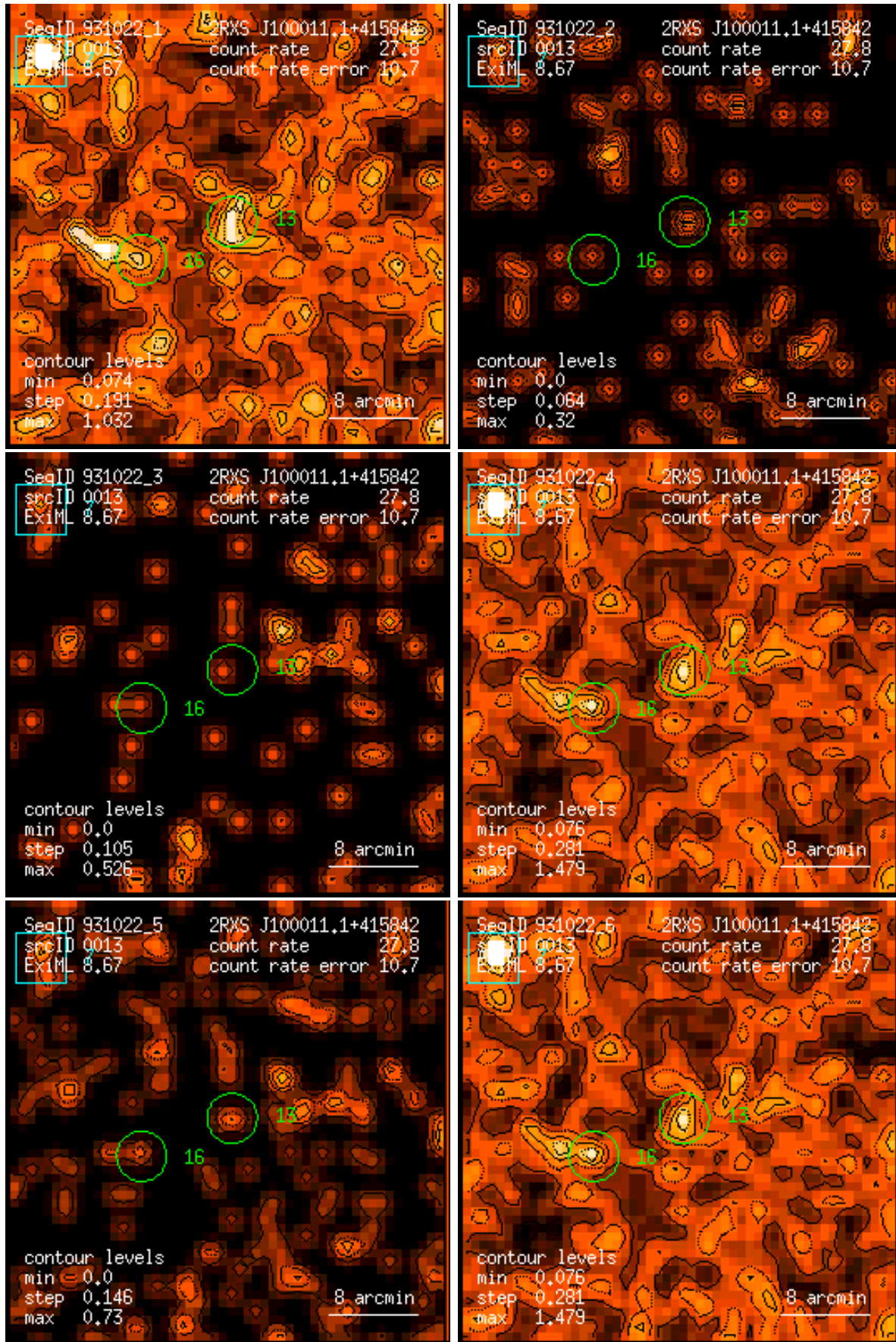
Figure 13: RASS 931022: detection 0013: band rate images, Gaussian filter: (1) PSPC channels 11 – 41, (2) 52 – 90, (3) 91 – 201, (4) 11 – 235, (5) 52 – 201, (6) 11 – 201. Broad band rates in counts/ks. Band rate contour levels in counts/ks/arcmin 2 .
