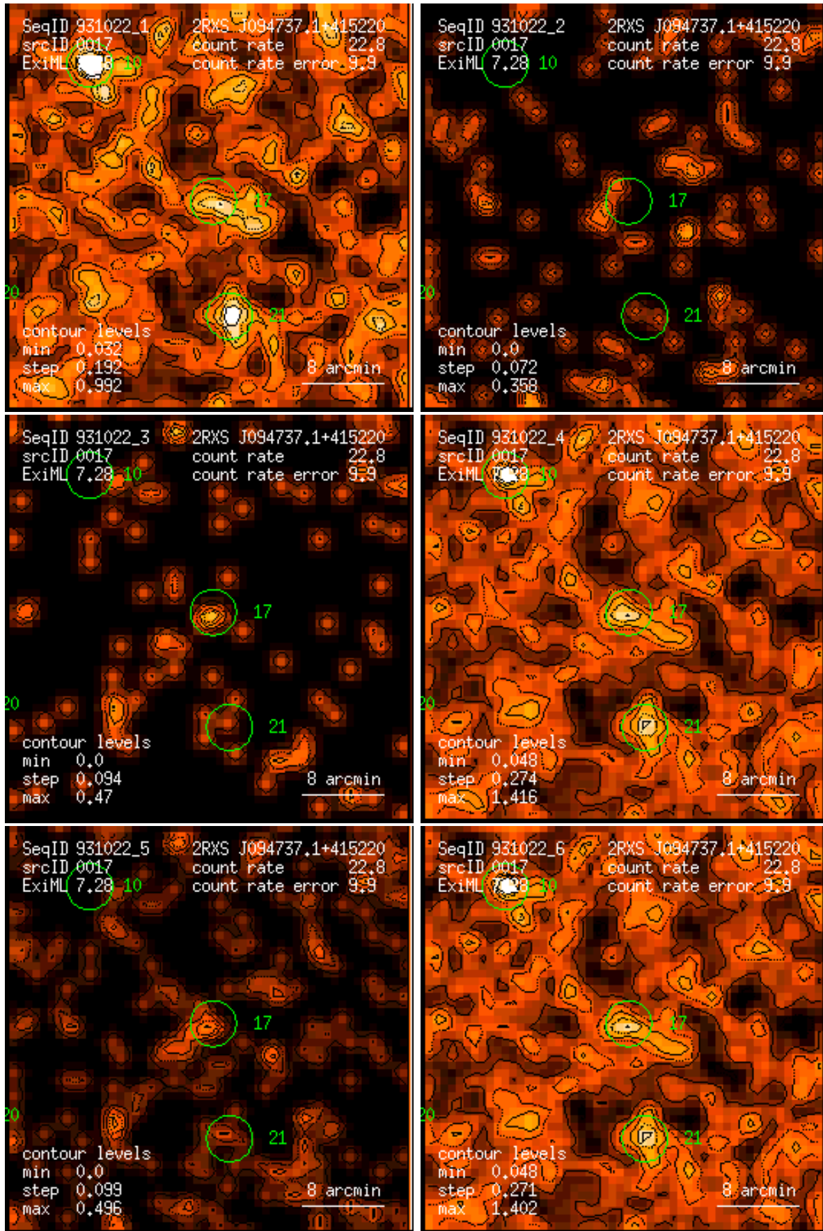
Figure 17: RASS 931022: detection 0017: band rate images, Gaussian filter: (1) PSPC channels 11 – 41, (2) 52 – 90, (3) 91 – 201, (4) 11 – 235, (5) 52 – 201, (6) 11 – 201. Broad band rates in counts/ks. Band rate contour levels in counts/ks/arcmin 2 .
