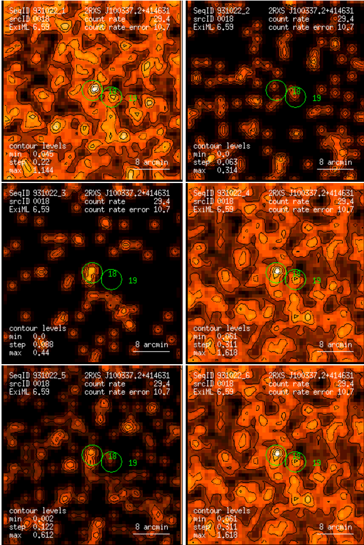
Figure 18: RASS 931022: detection 0018: band rate images, Gaussian filter: (1) PSPC channels 11 – 41, (2) 52 – 90, (3) 91 – 201, (4) 11 – 235, (5) 52 – 201, (6) 11 – 201. Broad band rates in counts/ks. Band rate contour levels in counts/ks/arcmin 2 .
