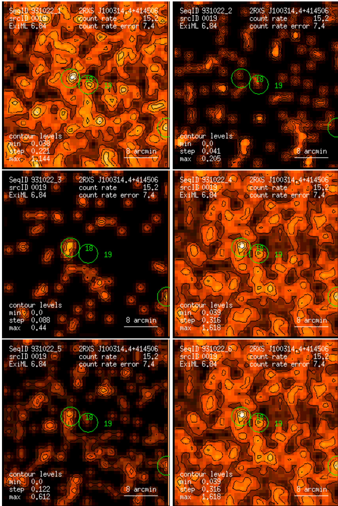
Figure 19: RASS 931022: detection 0019: band rate images, Gaussian filter: (1) PSPC channels 11 – 41, (2) 52 – 90, (3) 91 – 201, (4) 11 – 235, (5) 52 – 201, (6) 11 – 201. Broad band rates in counts/ks. Band rate contour levels in counts/ks/arcmin 2 .
