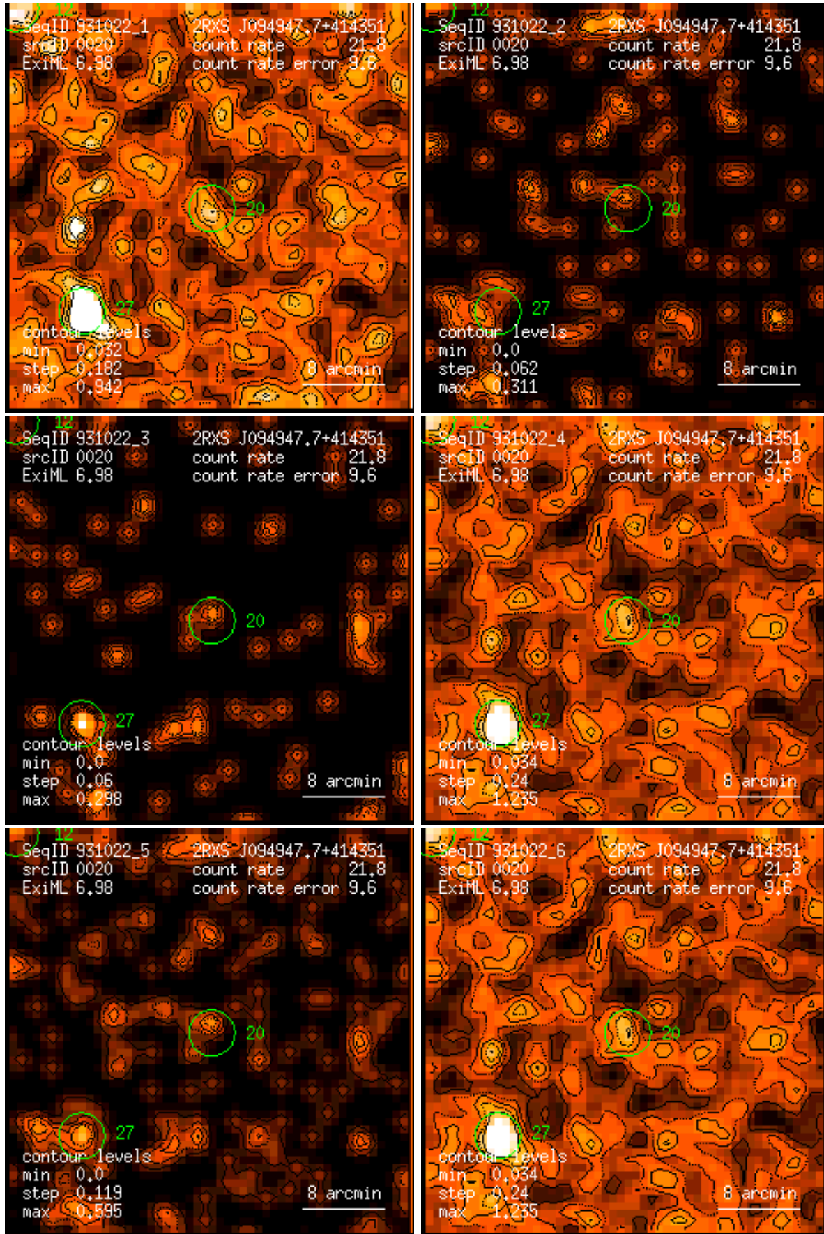
Figure 20: RASS 931022: detection 0020: band rate images, Gaussian filter: (1) PSPC channels 11 – 41, (2) 52 – 90, (3) 91 – 201, (4) 11 – 235, (5) 52 – 201, (6) 11 – 201. Broad band rates in counts/ks. Band rate contour levels in counts/ks/arcmin 2 .
