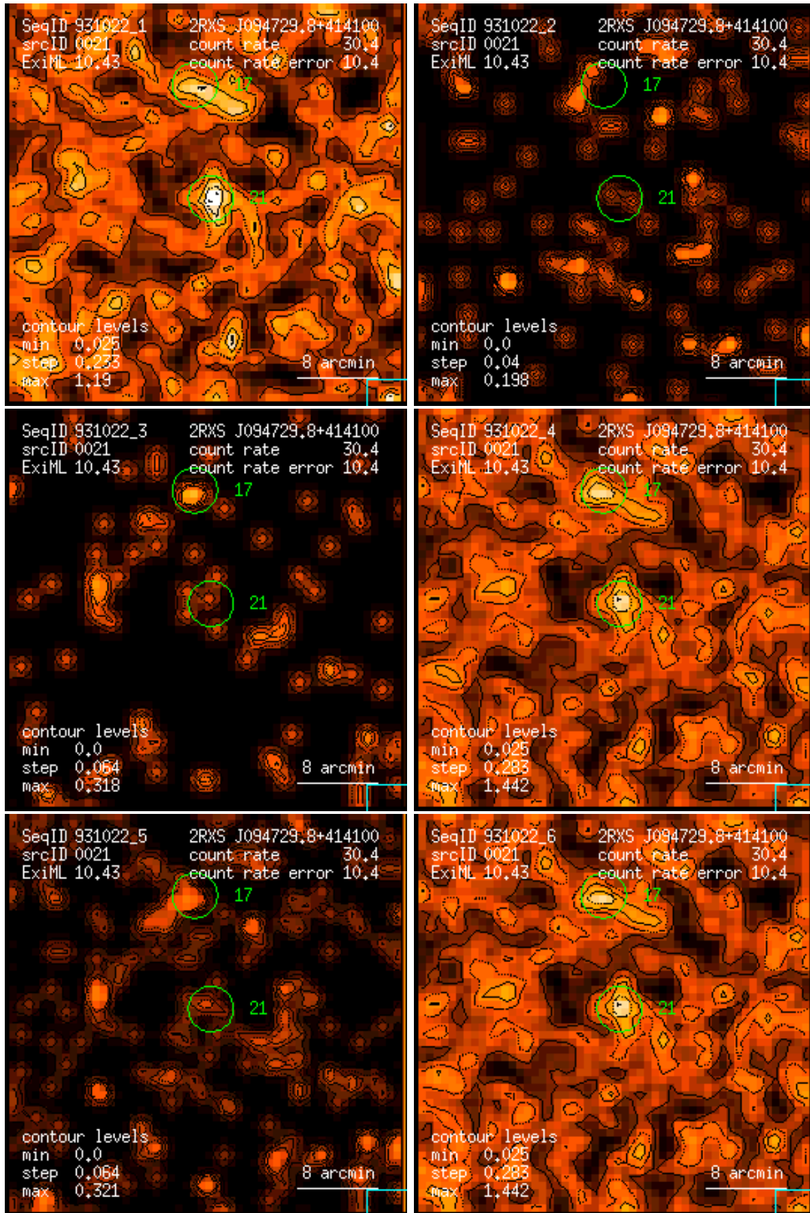
Figure 21: RASS 931022: detection 0021: band rate images, Gaussian filter: (1) PSPC channels 11 – 41, (2) 52 – 90, (3) 91 – 201, (4) 11 – 235, (5) 52 – 201, (6) 11 – 201. Broad band rates in counts/ks. Band rate contour levels in counts/ks/arcmin 2 .
