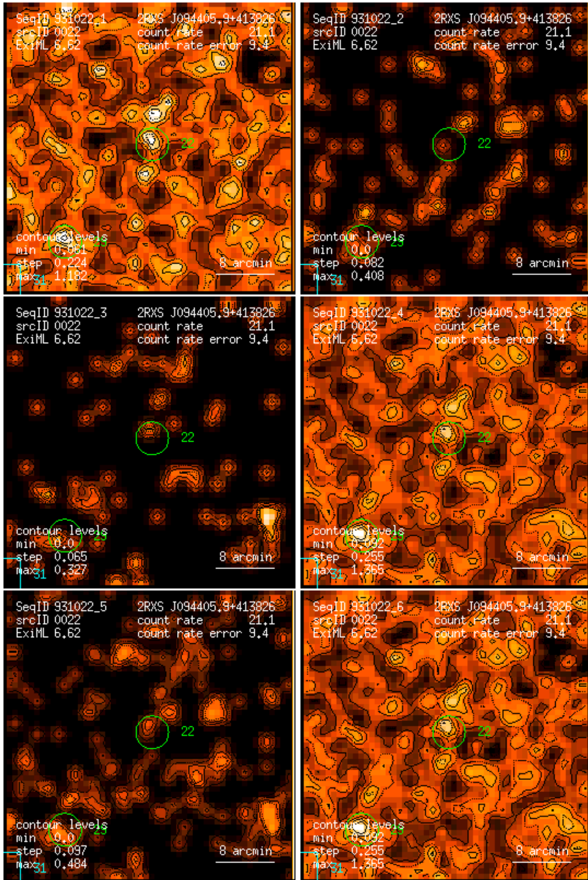
Figure 22: RASS 931022: detection 0022: band rate images, Gaussian filter: (1) PSPC channels 11 – 41, (2) 52 – 90, (3) 91 – 201, (4) 11 – 235, (5) 52 – 201, (6) 11 – 201. Broad band rates in counts/ks. Band rate contour levels in counts/ks/arcmin 2 .
