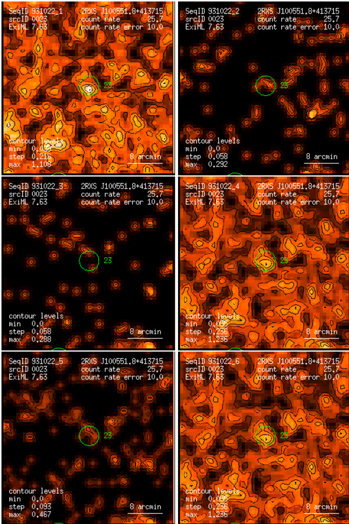
Figure 23: RASS 931022: detection 0023: band rate images, Gaussian filter: (1) PSPC channels 11 – 41, (2) 52 – 90, (3) 91 – 201, (4) 11 – 235, (5) 52 – 201, (6) 11 – 201. Broad band rates in counts/ks. Band rate contour levels in counts/ks/arcmin 2 .
