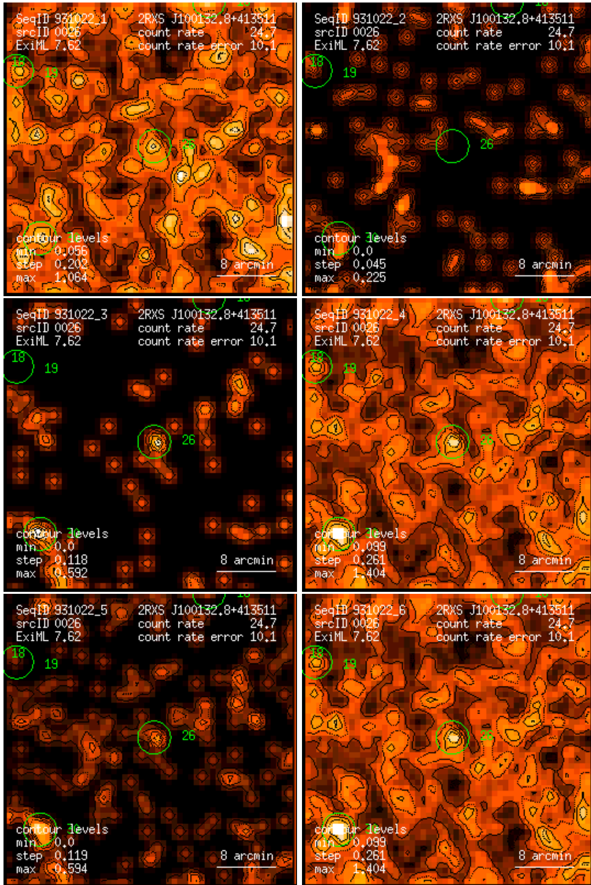
Figure 26: RASS 931022: detection 0026: band rate images, Gaussian filter: (1) PSPC channels 11 – 41, (2) 52 – 90, (3) 91 – 201, (4) 11 – 235, (5) 52 – 201, (6) 11 – 201. Broad band rates in counts/ks. Band rate contour levels in counts/ks/arcmin 2 .
