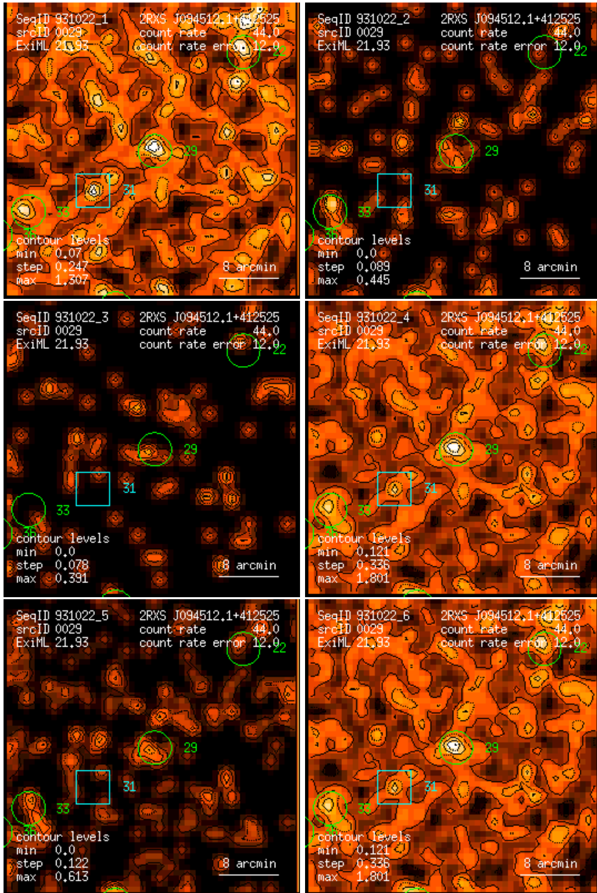
Figure 29: RASS 931022: detection 0029: band rate images, Gaussian filter: (1) PSPC channels 11 – 41, (2) 52 – 90, (3) 91 – 201, (4) 11 – 235, (5) 52 – 201, (6) 11 – 201. Broad band rates in counts/ks. Band rate contour levels in counts/ks/arcmin 2 .
