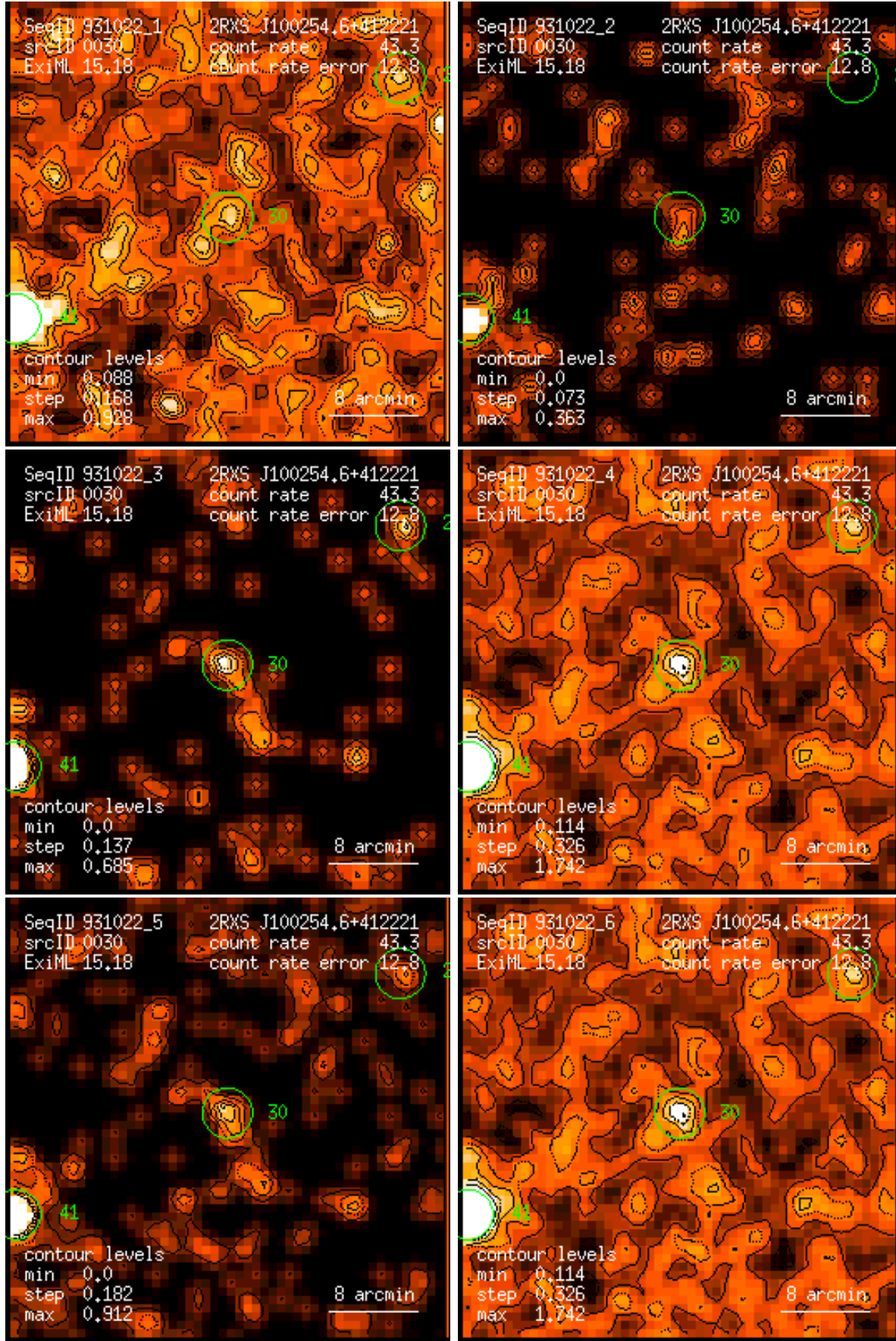
Figure 30: RASS 931022: detection 0030: band rate images, Gaussian filter: (1) PSPC channels 11 – 41, (2) 52 – 90, (3) 91 – 201, (4) 11 – 235, (5) 52 – 201, (6) 11 – 201. Broad band rates in counts/ks. Band rate contour levels in counts/ks/arcmin 2 .
