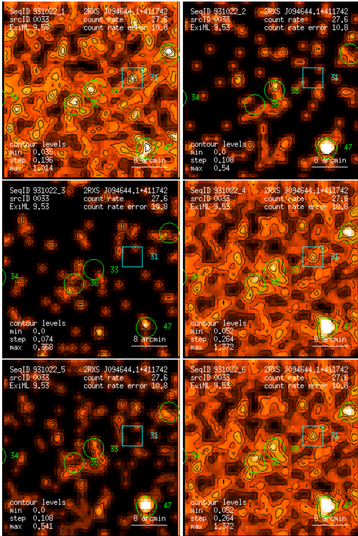
Figure 33: RASS 931022: detection 0033: band rate images, Gaussian filter: (1) PSPC channels 11 – 41, (2) 52 – 90, (3) 91 – 201, (4) 11 – 235, (5) 52 – 201, (6) 11 – 201. Broad band rates in counts/ks. Band rate contour levels in counts/ks/arcmin 2 .
