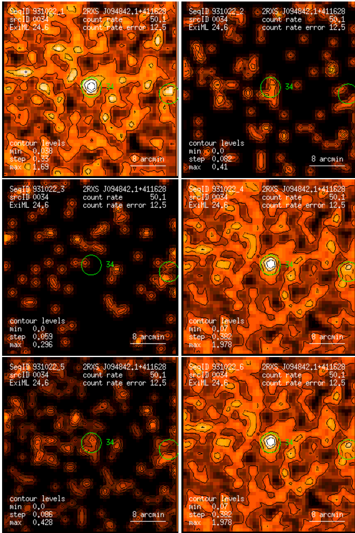
Figure 34: RASS 931022: detection 0034: band rate images, Gaussian filter: (1) PSPC channels 11 – 41, (2) 52 – 90, (3) 91 – 201, (4) 11 – 235, (5) 52 – 201, (6) 11 – 201. Broad band rates in counts/ks. Band rate contour levels in counts/ks/arcmin 2 .
