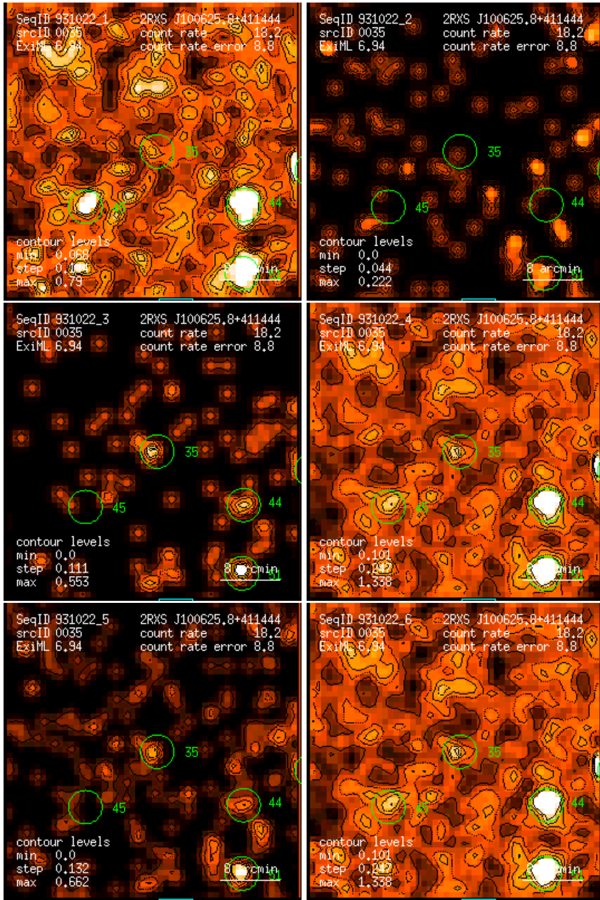
Figure 35: RASS 931022: detection 0035: band rate images, Gaussian filter: (1) PSPC channels 11 – 41, (2) 52 – 90, (3) 91 – 201, (4) 11 – 235, (5) 52 – 201, (6) 11 – 201. Broad band rates in counts/ks. Band rate contour levels in counts/ks/arcmin 2 .
