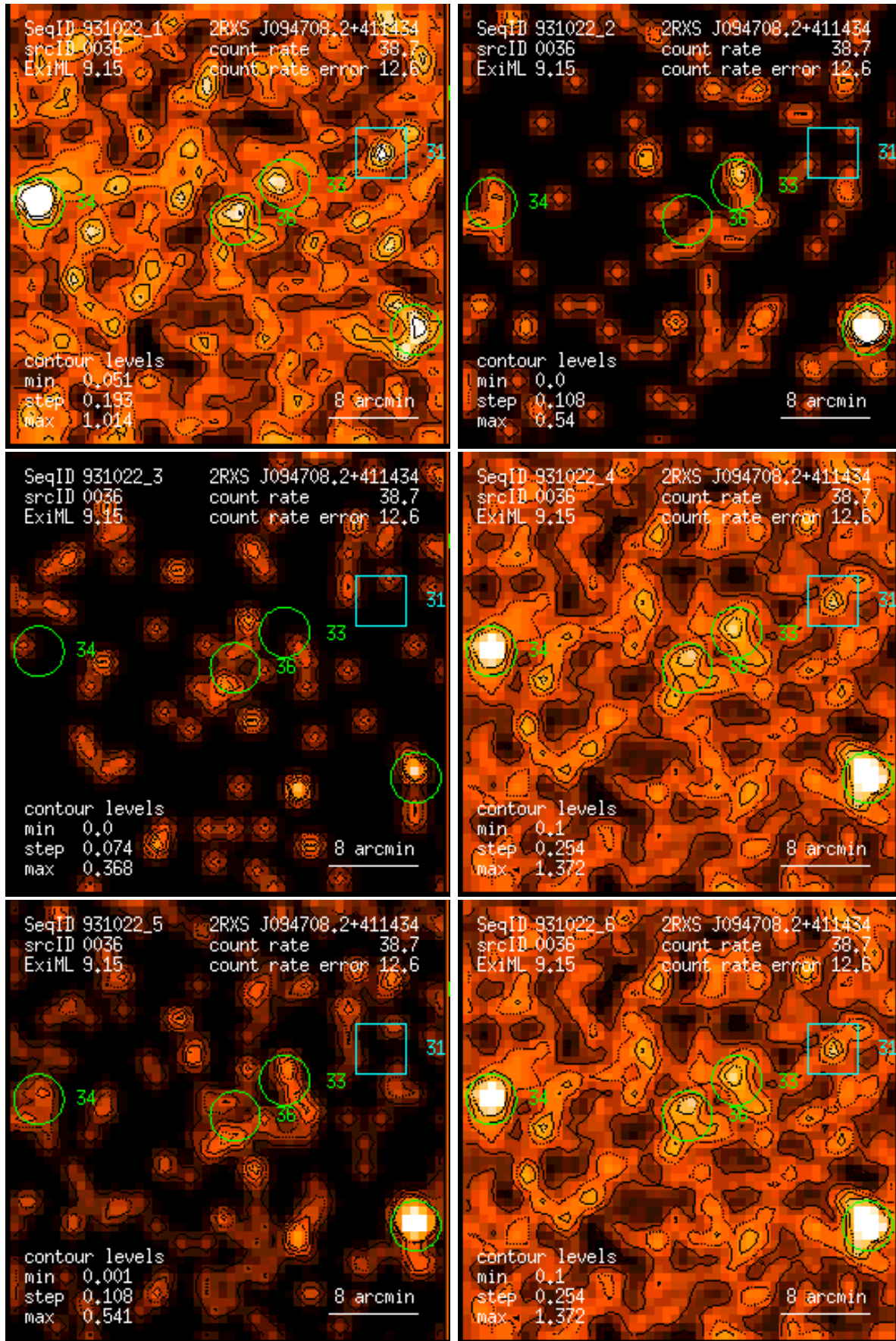
Figure 36: RASS 931022: detection 0036: band rate images, Gaussian filter: (1) PSPC channels 11 – 41, (2) 52 – 90, (3) 91 – 201, (4) 11 – 235, (5) 52 – 201, (6) 11 – 201. Broad band rates in counts/ks. Band rate contour levels in counts/ks/arcmin 2 .
