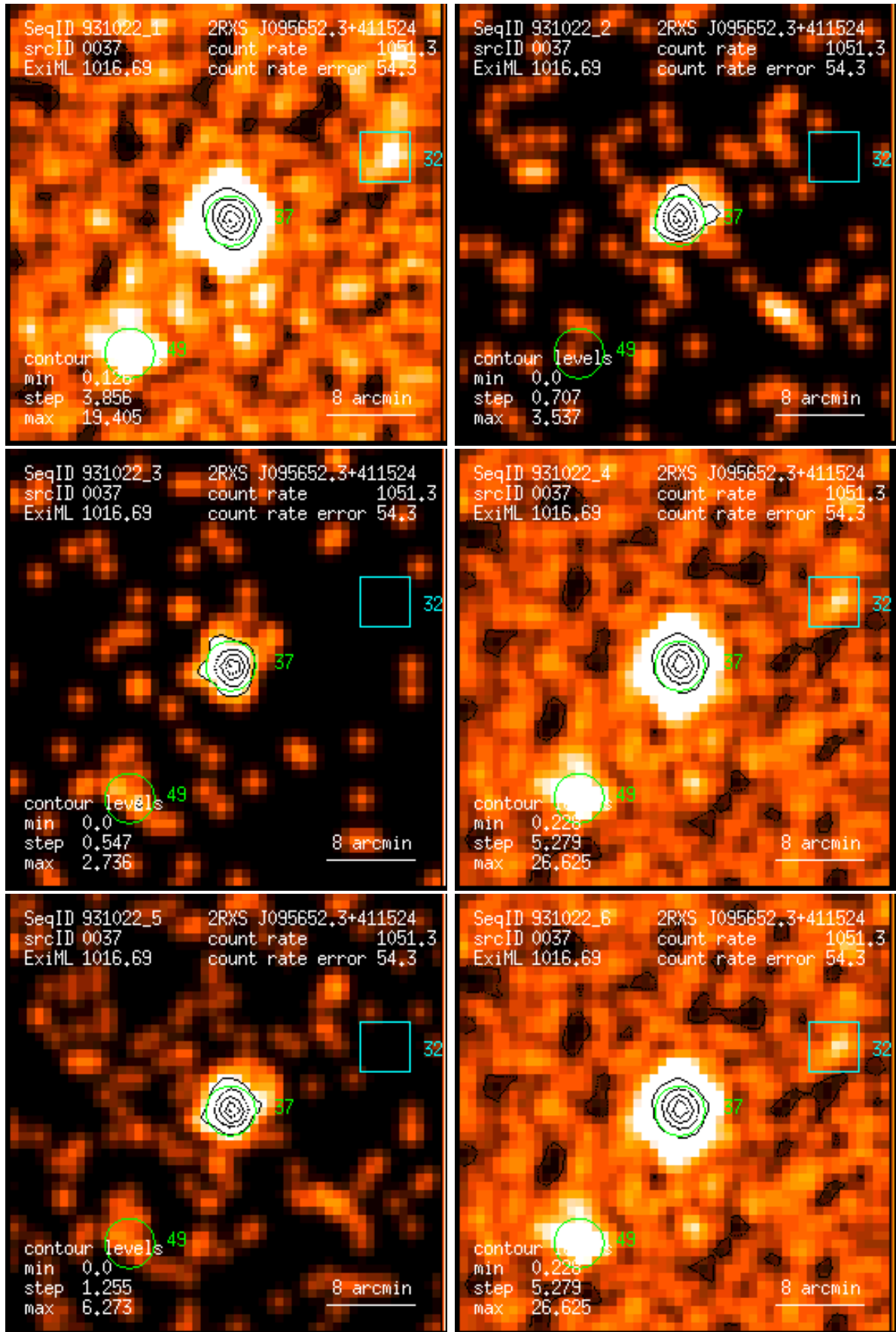
Figure 37: RASS 931022: detection 0037: band rate images, Gaussian filter: (1) PSPC channels 11 – 41, (2) 52 – 90, (3) 91 – 201, (4) 11 – 235, (5) 52 – 201, (6) 11 – 201. Broad band rates in counts/ks. Band rate contour levels in counts/ks/arcmin 2 .
