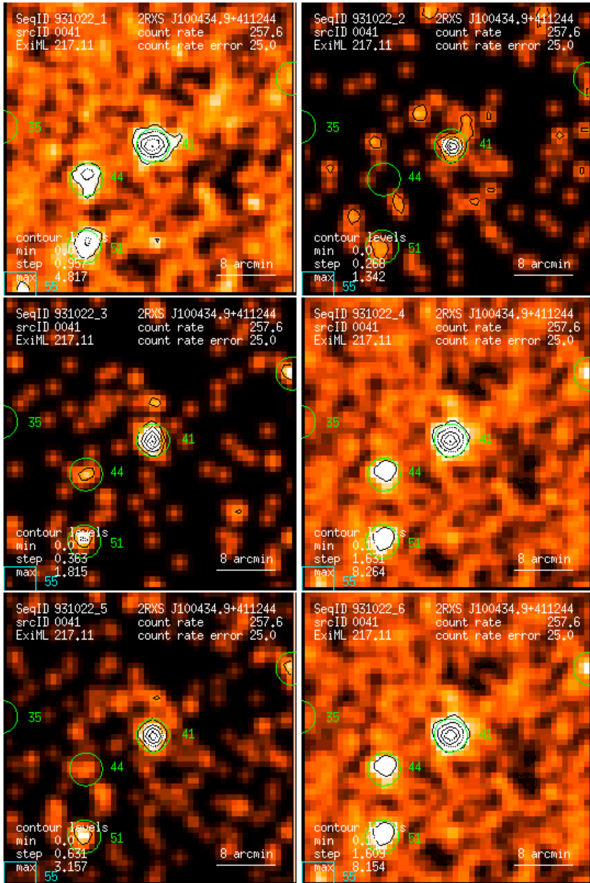
Figure 41: RASS 931022: detection 0041: band rate images, Gaussian filter: (1) PSPC channels 11 – 41, (2) 52 – 90, (3) 91 – 201, (4) 11 – 235, (5) 52 – 201, (6) 11 – 201. Broad band rates in counts/ks. Band rate contour levels in counts/ks/arcmin 2 .
