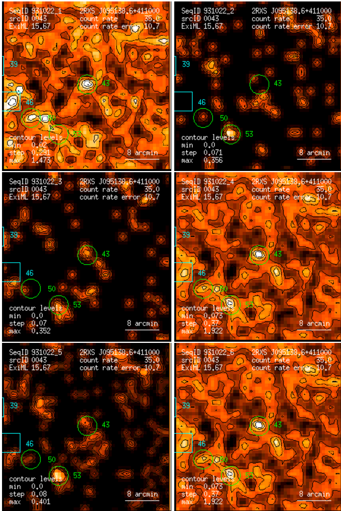
Figure 43: RASS 931022: detection 0043: band rate images, Gaussian filter: (1) PSPC channels 11 – 41, (2) 52 – 90, (3) 91 – 201, (4) 11 – 235, (5) 52 – 201, (6) 11 – 201. Broad band rates in counts/ks. Band rate contour levels in counts/ks/arcmin 2 .
