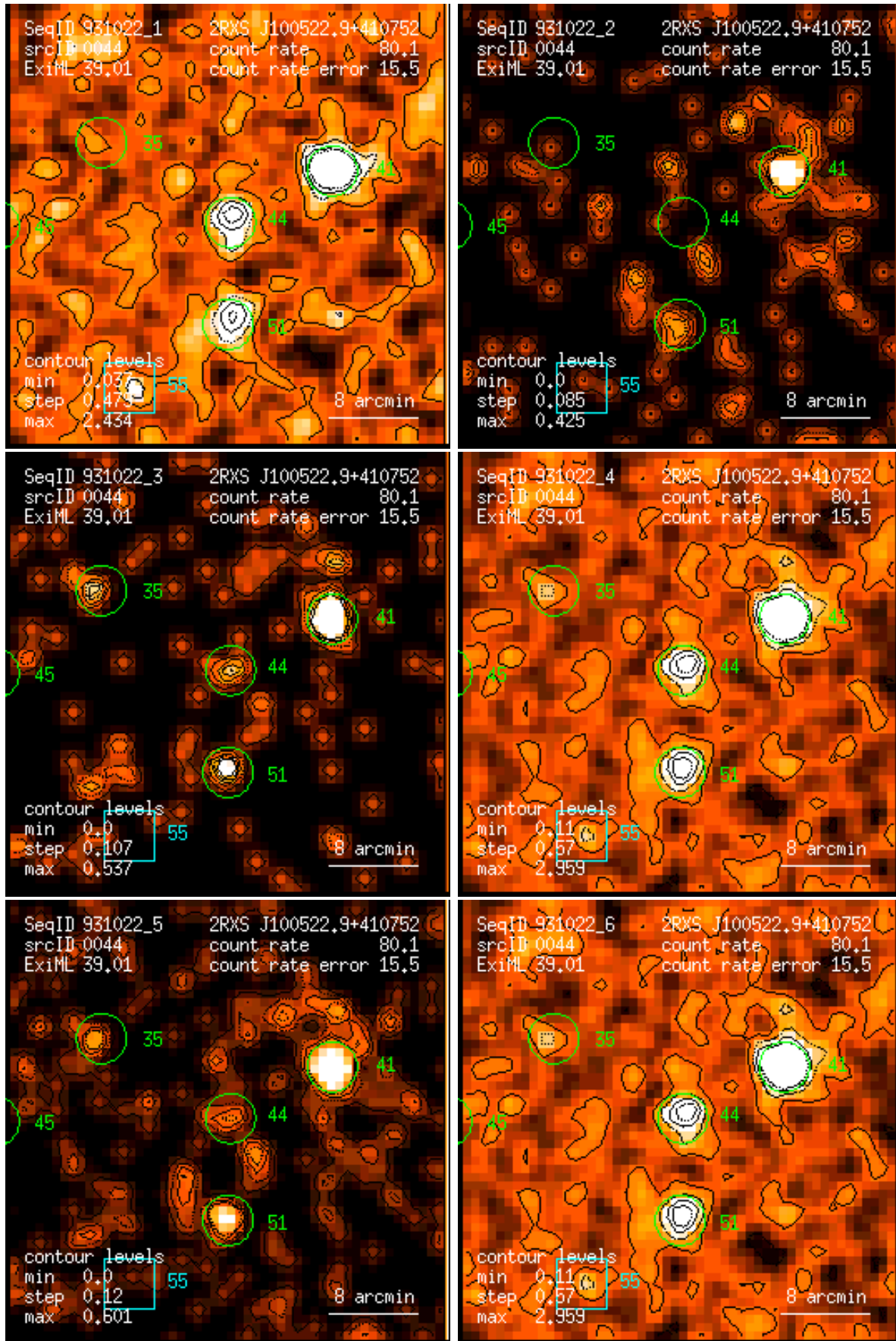
Figure 44: RASS 931022: detection 0044: band rate images, Gaussian filter: (1) PSPC channels 11 – 41, (2) 52 – 90, (3) 91 – 201, (4) 11 – 235, (5) 52 – 201, (6) 11 – 201. Broad band rates in counts/ks. Band rate contour levels in counts/ks/arcmin 2 .
