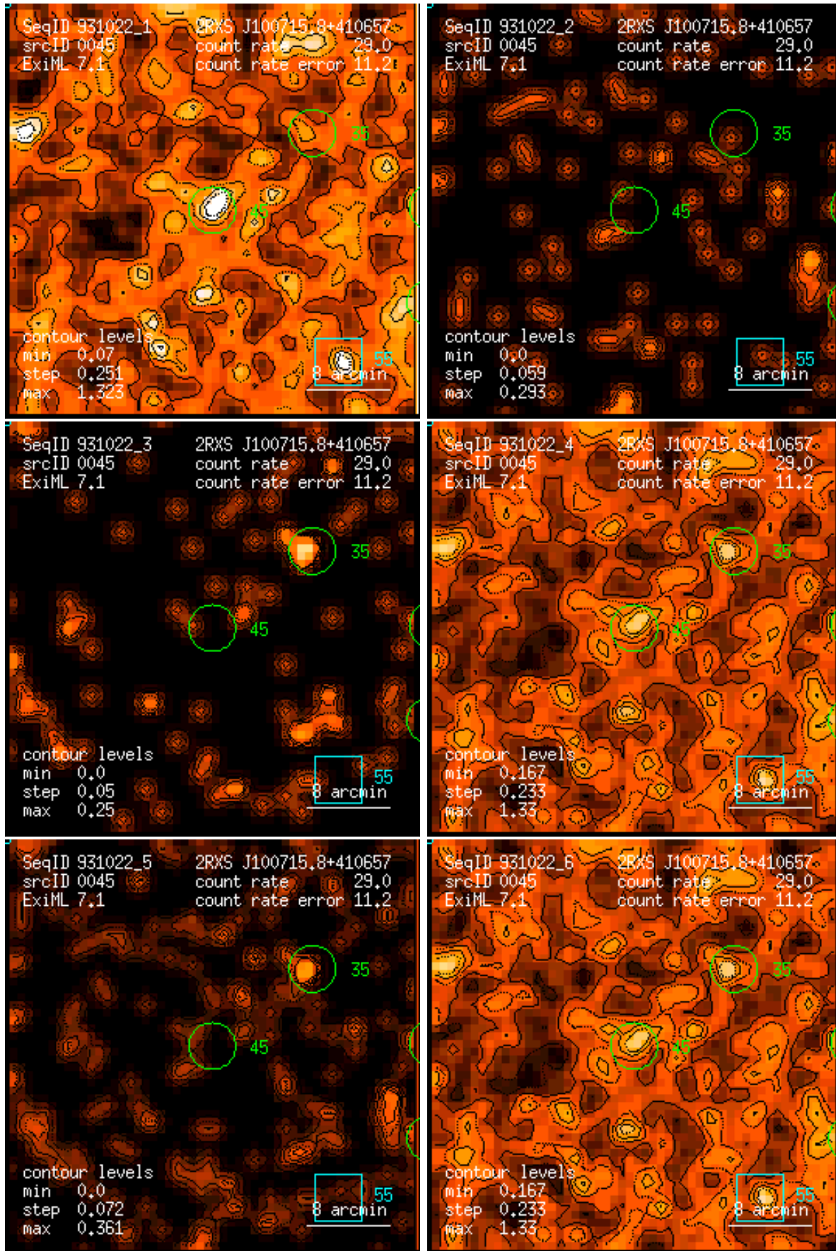
Figure 45: RASS 931022: detection 0045: band rate images, Gaussian filter: (1) PSPC channels 11 – 41, (2) 52 – 90, (3) 91 – 201, (4) 11 – 235, (5) 52 – 201, (6) 11 – 201. Broad band rates in counts/ks. Band rate contour levels in counts/ks/arcmin 2 .
