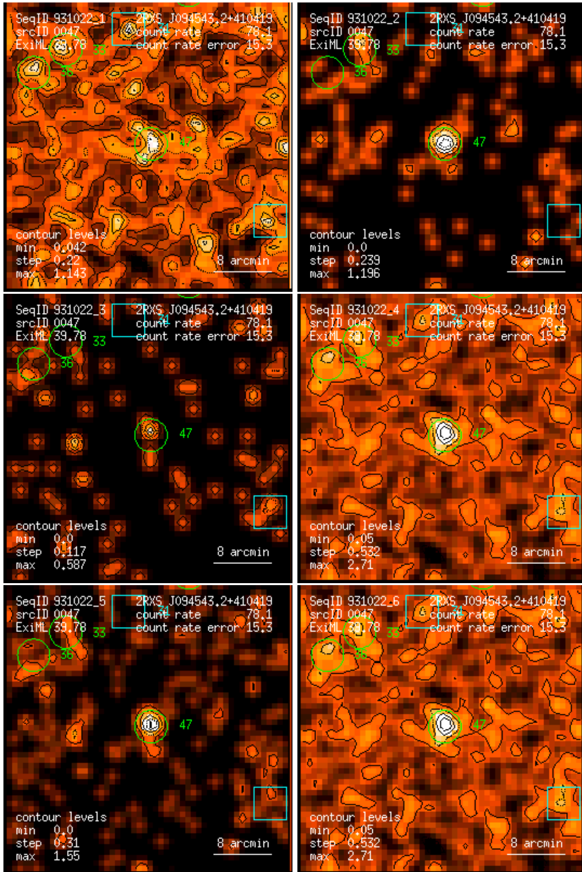
Figure 47: RASS 931022: detection 0047: band rate images, Gaussian filter: (1) PSPC channels 11 – 41, (2) 52 – 90, (3) 91 – 201, (4) 11 – 235, (5) 52 – 201, (6) 11 – 201. Broad band rates in counts/ks. Band rate contour levels in counts/ks/arcmin 2 .
