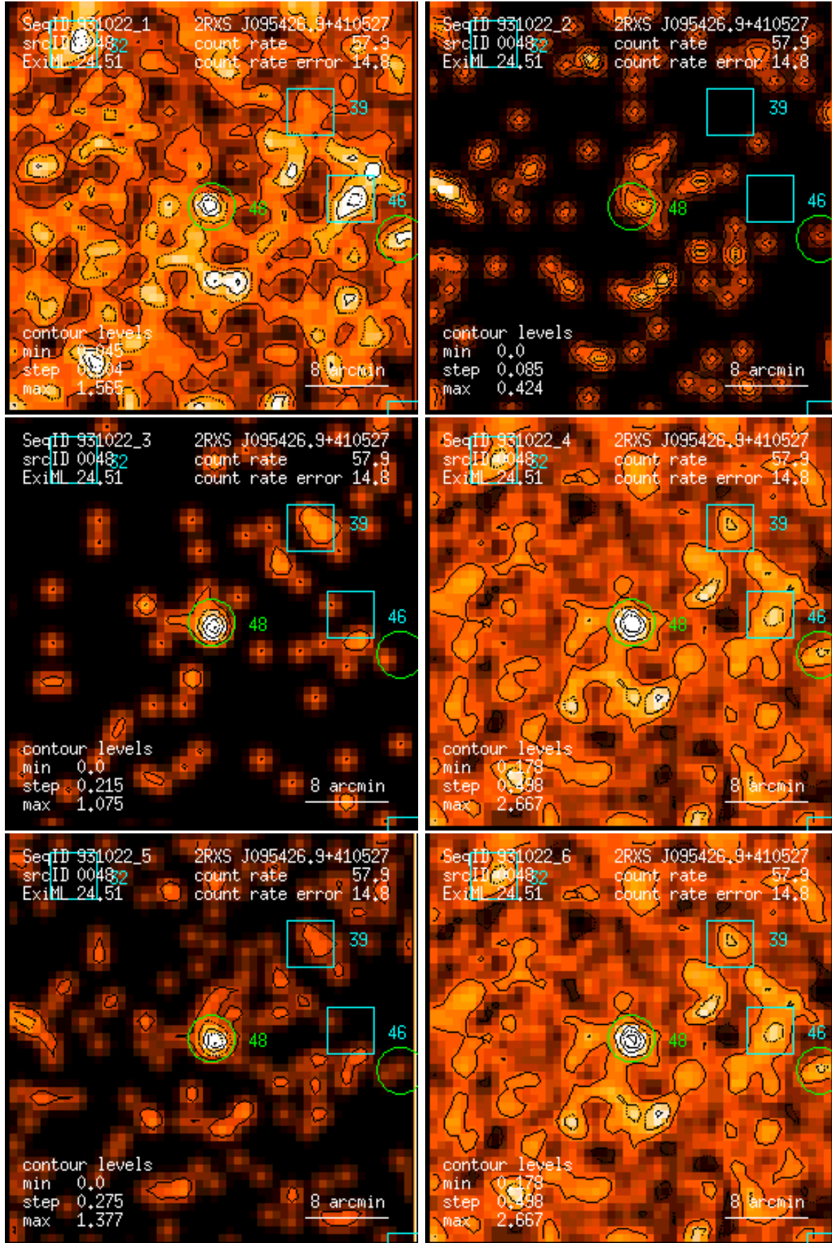
Figure 48: RASS 931022: detection 0048: band rate images, Gaussian filter: (1) PSPC channels 11 – 41, (2) 52 – 90, (3) 91 – 201, (4) 11 – 235, (5) 52 – 201, (6) 11 – 201. Broad band rates in counts/ks. Band rate contour levels in counts/ks/arcmin 2 .
