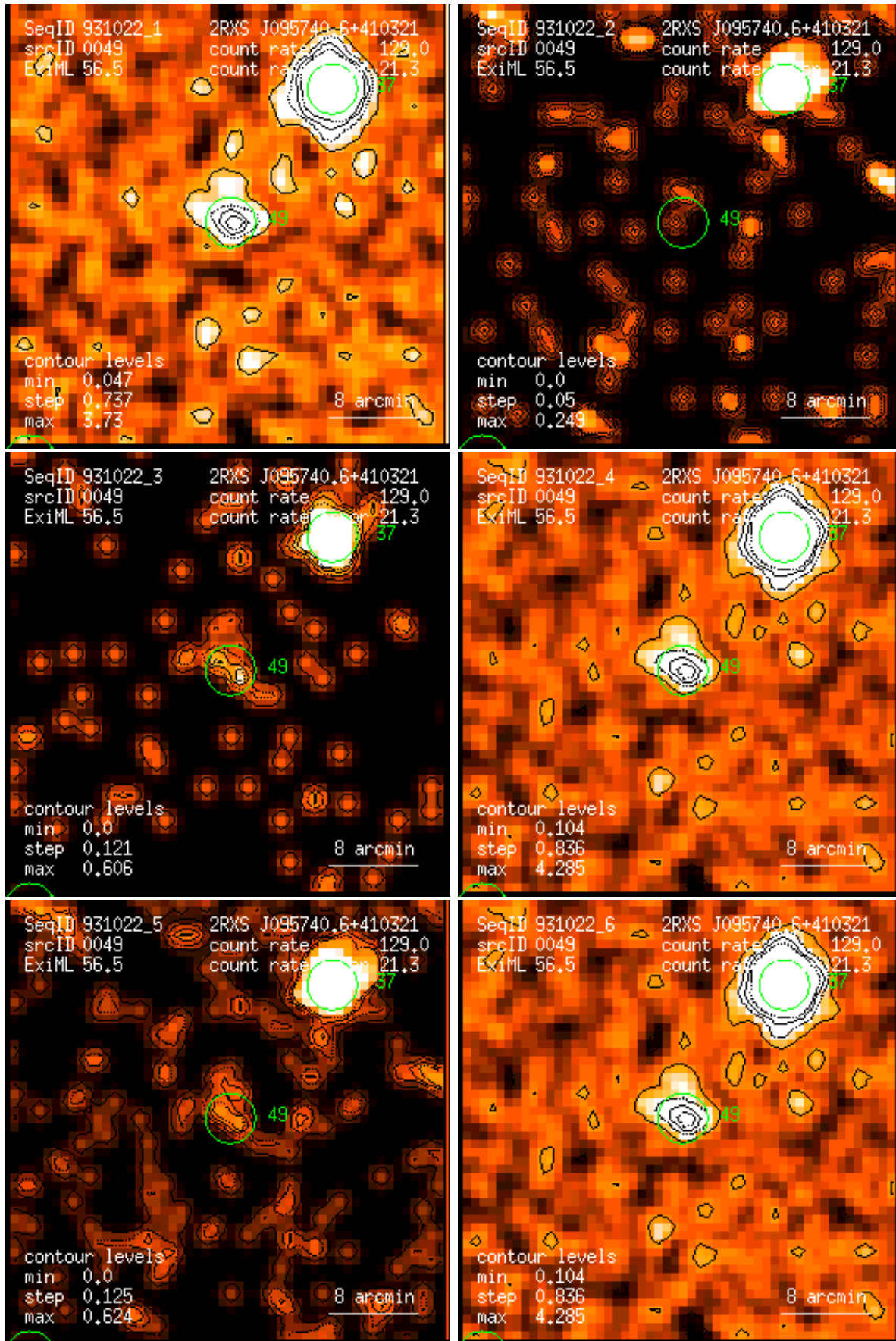
Figure 49: RASS 931022: detection 0049: band rate images, Gaussian filter: (1) PSPC channels 11 – 41, (2) 52 – 90, (3) 91 – 201, (4) 11 – 235, (5) 52 – 201, (6) 11 – 201. Broad band rates in counts/ks. Band rate contour levels in counts/ks/arcmin 2 .
