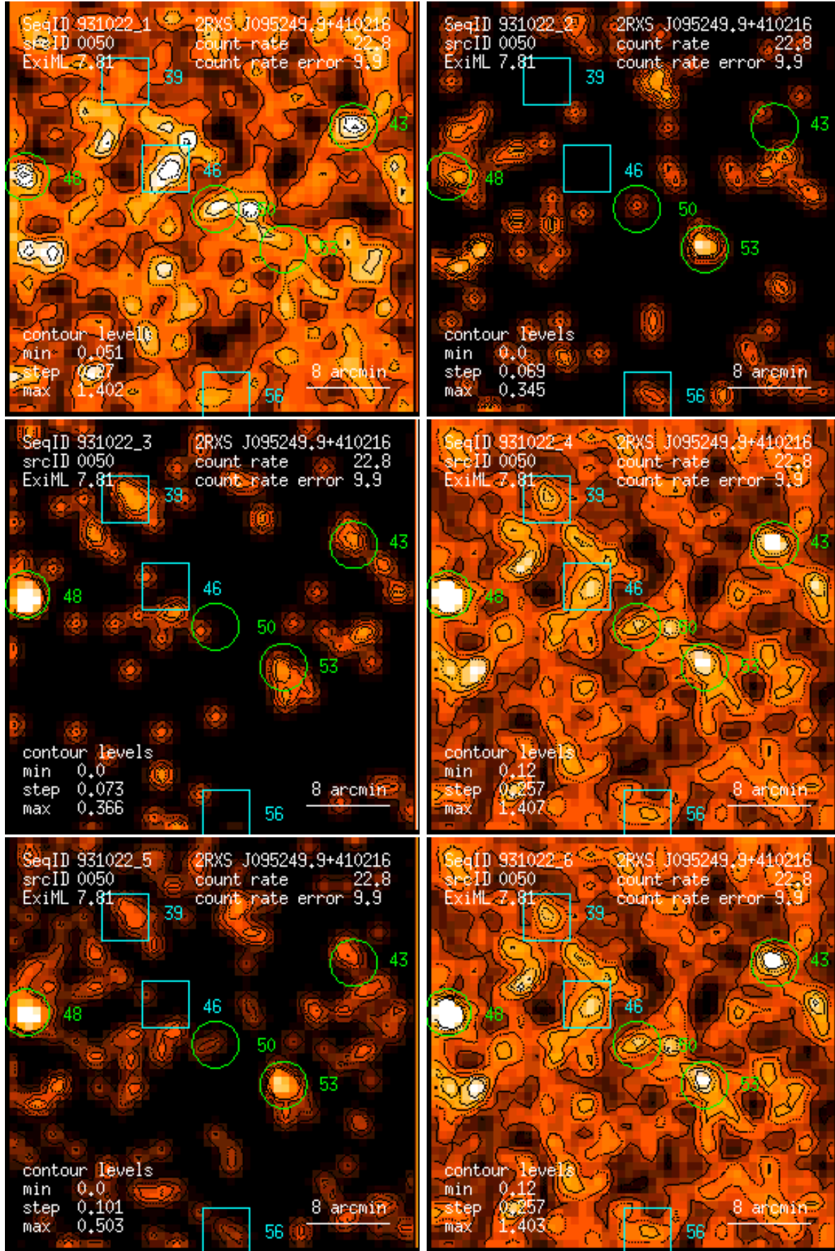
Figure 50: RASS 931022: detection 0050: band rate images, Gaussian filter: (1) PSPC channels 11 – 41, (2) 52 – 90, (3) 91 – 201, (4) 11 – 235, (5) 52 – 201, (6) 11 – 201. Broad band rates in counts/ks. Band rate contour levels in counts/ks/arcmin 2 .
