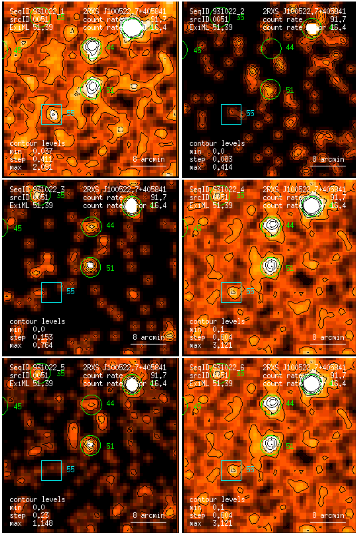
Figure 51: RASS 931022: detection 0051: band rate images, Gaussian filter: (1) PSPC channels 11 – 41, (2) 52 – 90, (3) 91 – 201, (4) 11 – 235, (5) 52 – 201, (6) 11 – 201. Broad band rates in counts/ks. Band rate contour levels in counts/ks/arcmin 2 .
