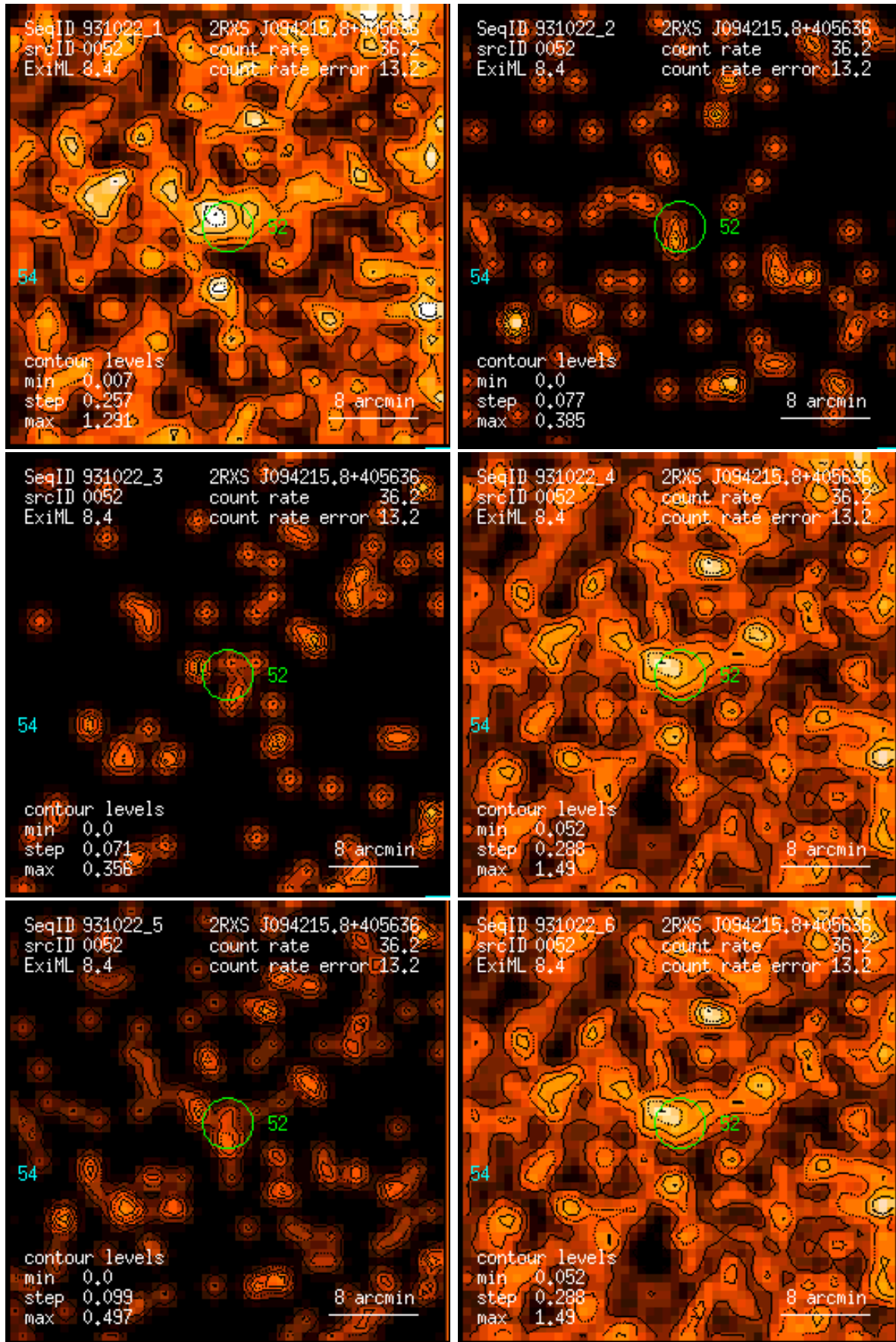
Figure 52: RASS 931022: detection 0052: band rate images, Gaussian filter: (1) PSPC channels 11 – 41, (2) 52 – 90, (3) 91 – 201, (4) 11 – 235, (5) 52 – 201, (6) 11 – 201. Broad band rates in counts/ks. Band rate contour levels in counts/ks/arcmin 2 .
