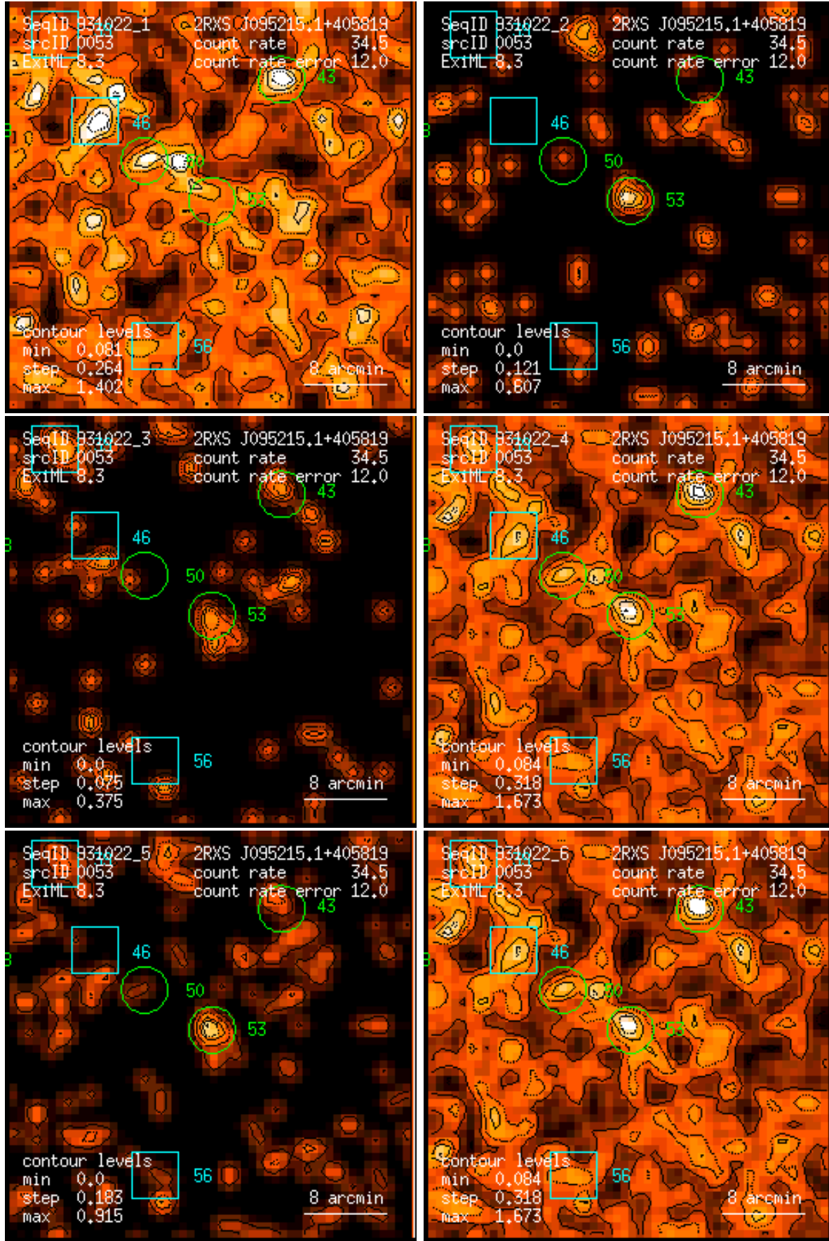
Figure 53: RASS 931022: detection 0053: band rate images, Gaussian filter: (1) PSPC channels 11 – 41, (2) 52 – 90, (3) 91 – 201, (4) 11 – 235, (5) 52 – 201, (6) 11 – 201. Broad band rates in counts/ks. Band rate contour levels in counts/ks/arcmin 2 .
