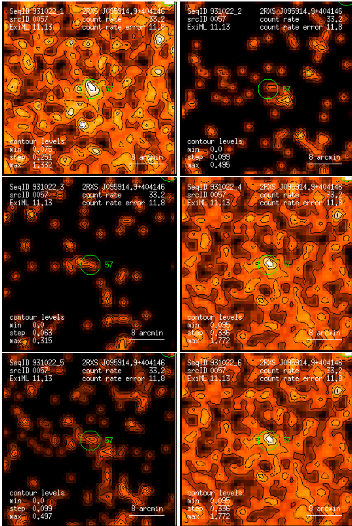
Figure 57: RASS 931022: detection 0057: band rate images, Gaussian filter: (1) PSPC channels 11 – 41, (2) 52 – 90, (3) 91 – 201, (4) 11 – 235, (5) 52 – 201, (6) 11 – 201. Broad band rates in counts/ks. Band rate contour levels in counts/ks/arcmin 2 .
